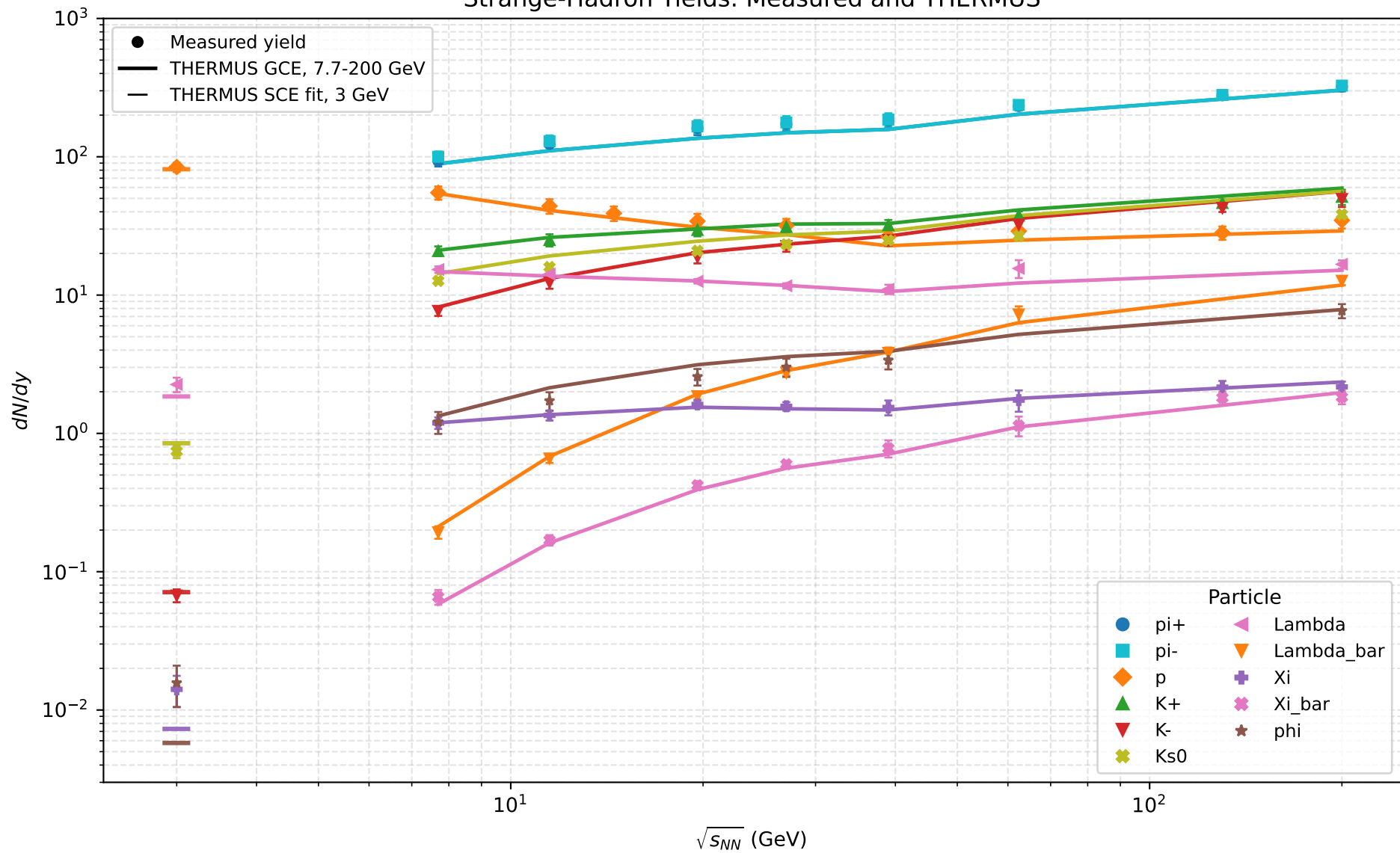
Strange-Hadron Yields: Measured and THERMUS
