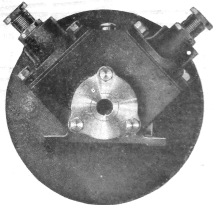
Air pressure pump—Assembled views
