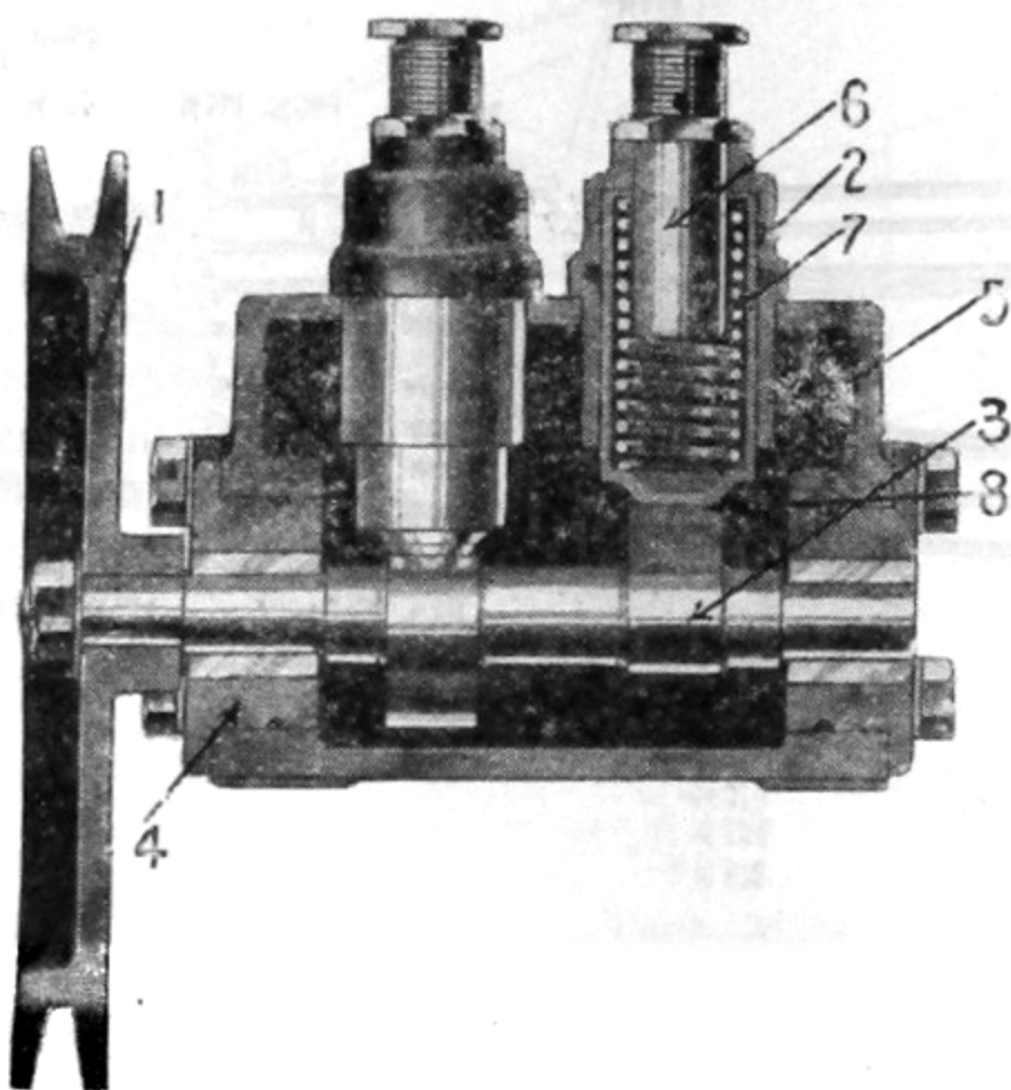
Air pressure pump—Assembled views
