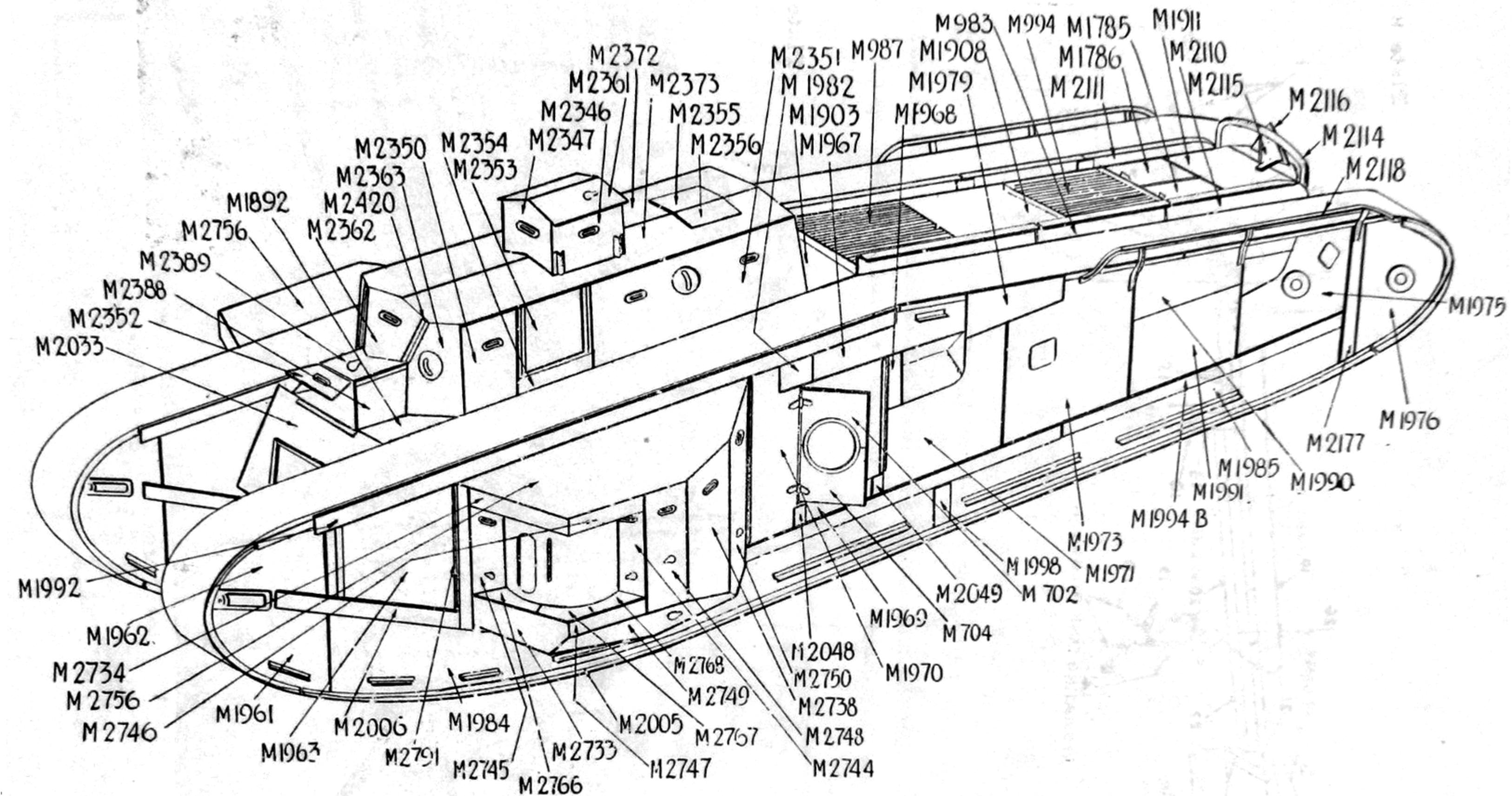
Tank, Mark VIII—Assembled view (showing armor)
