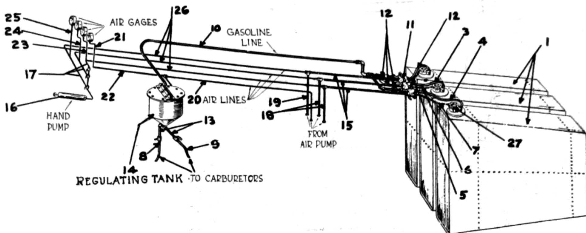
Gasoline tanks with pressure system—Assembled view
