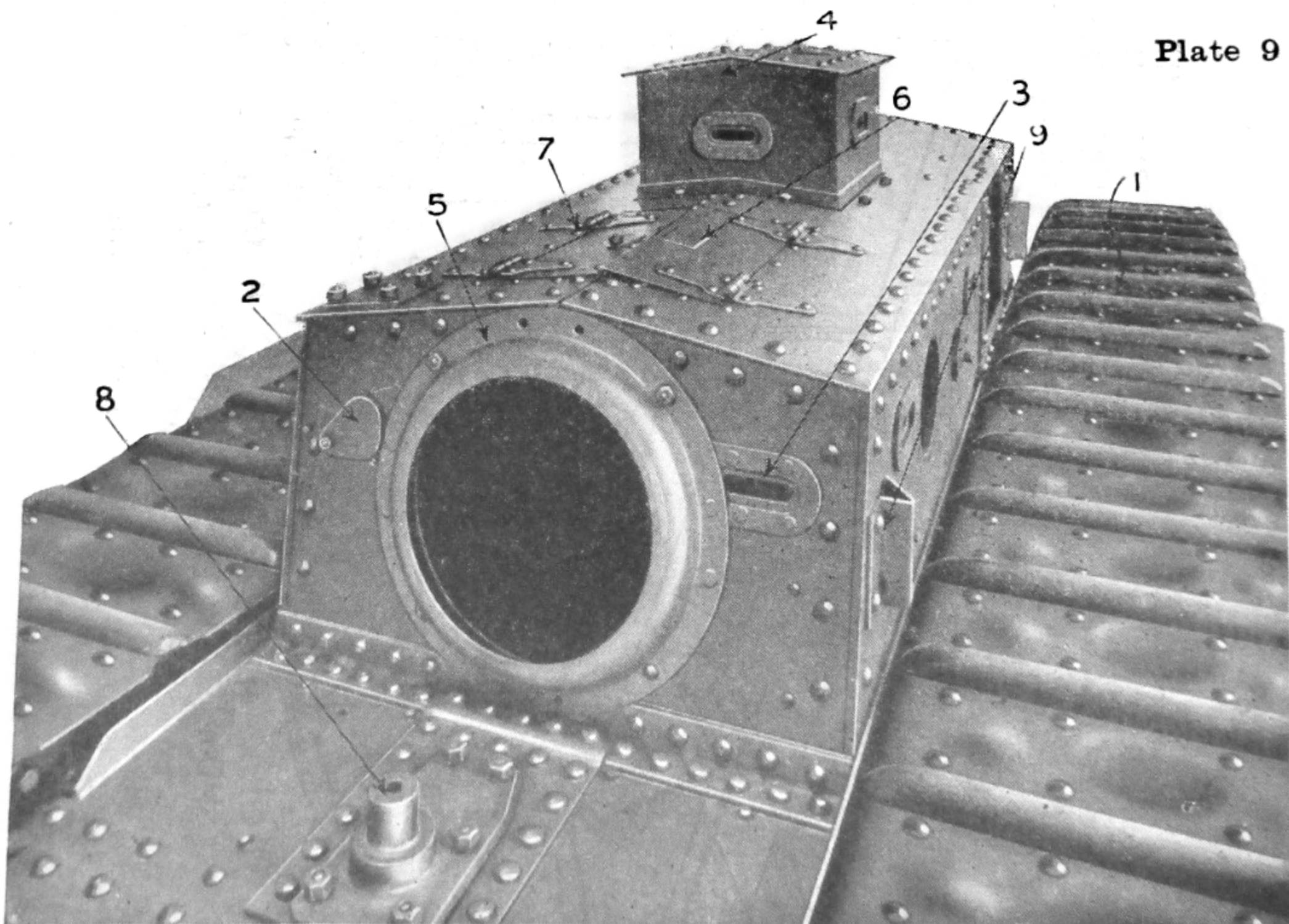
Main turret—Assembled view
