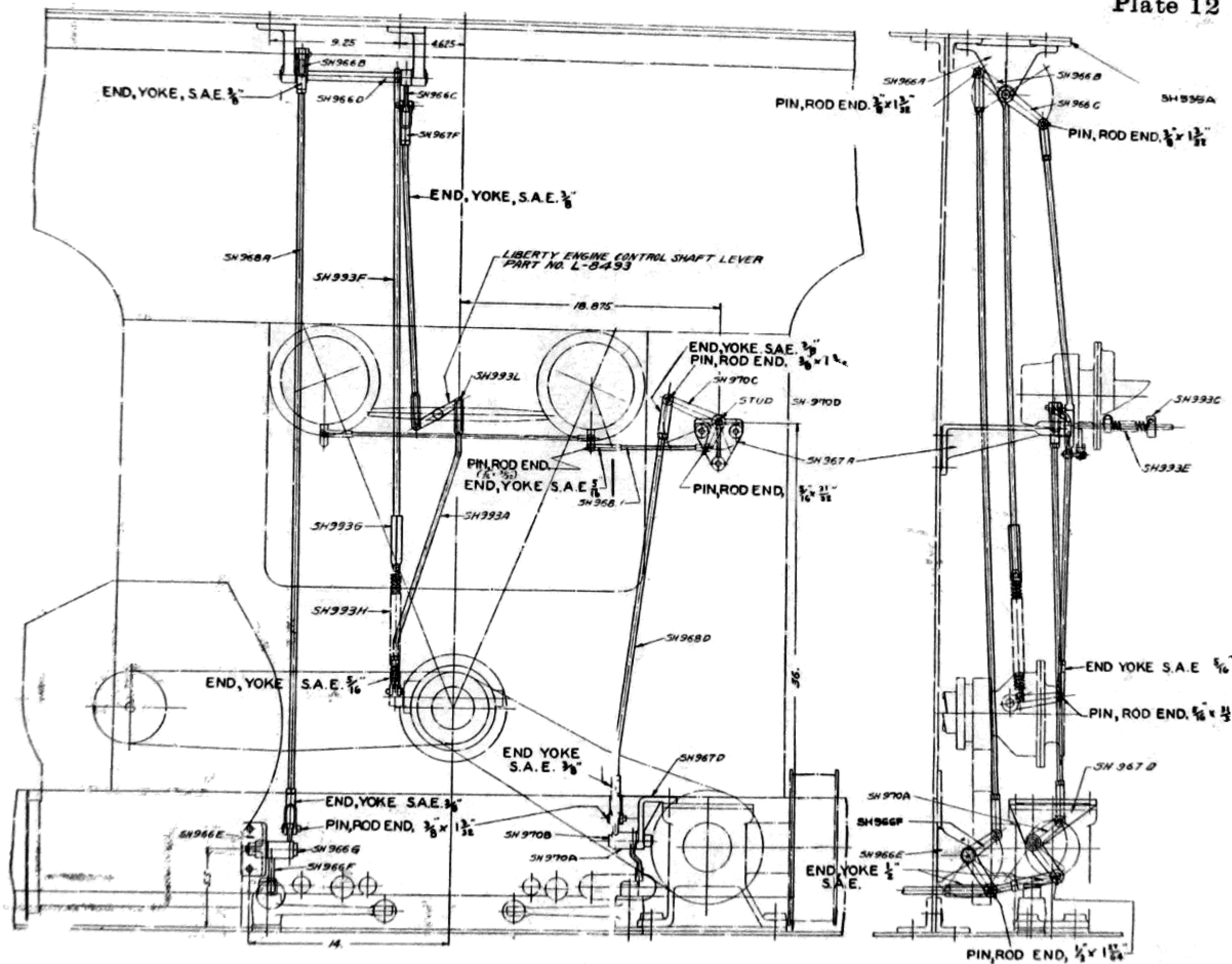
Engine control rods—Assembled view
