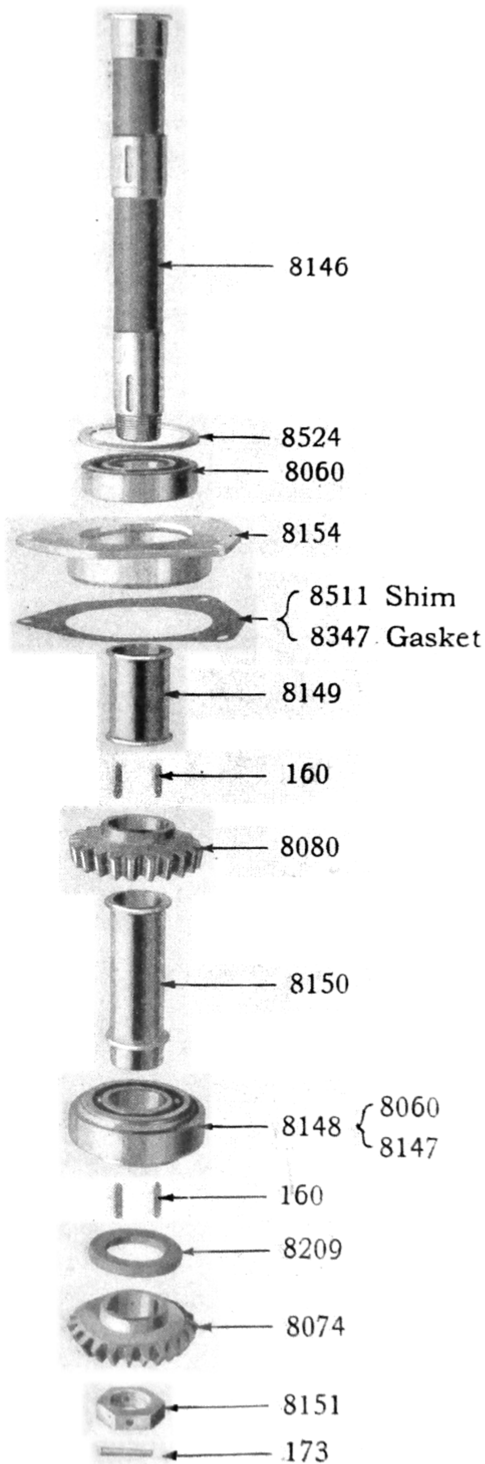
Generator drive shaft—Parts
