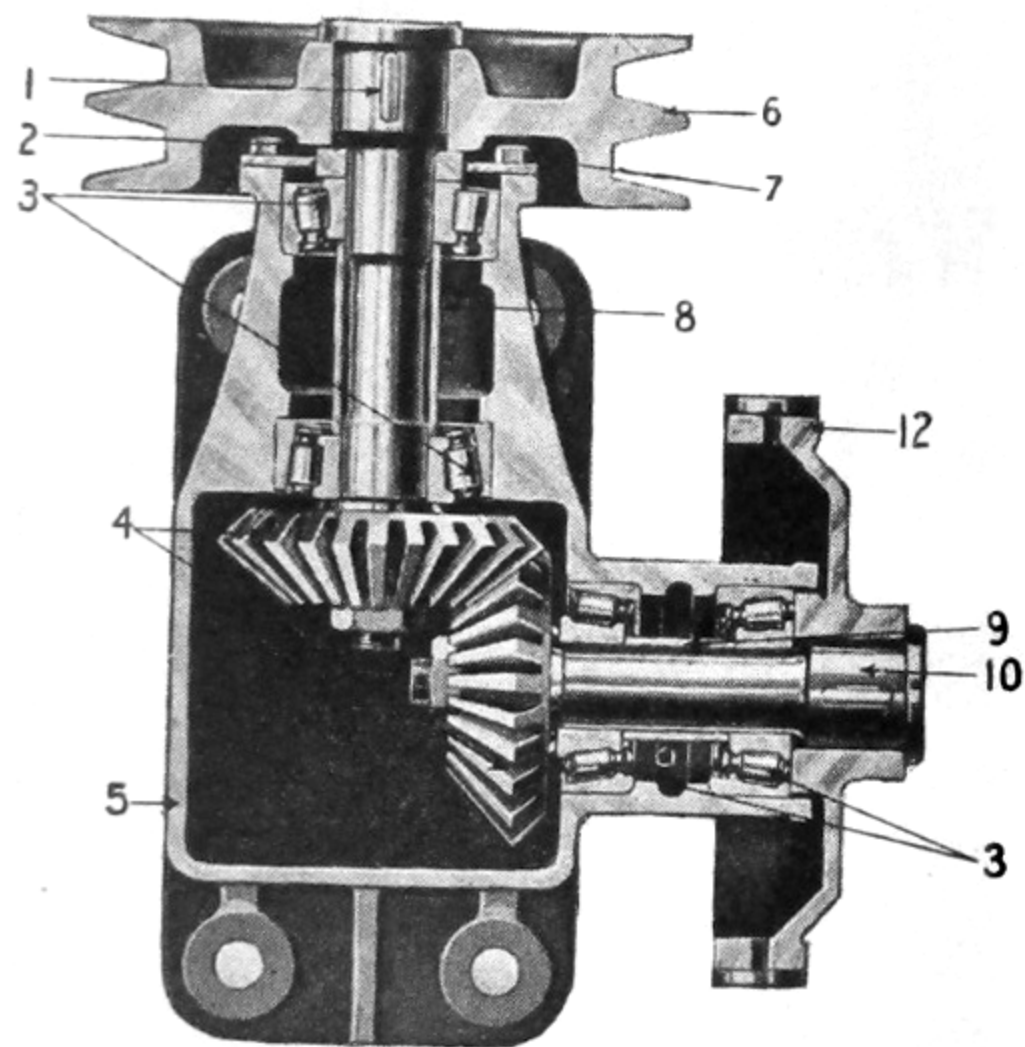
Fan bevel box—Assembled view (pulley shown now substituted by new design)
