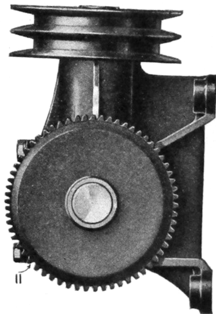
Fan bevel box—Assembled view (pulley shown now substituted by new design)
