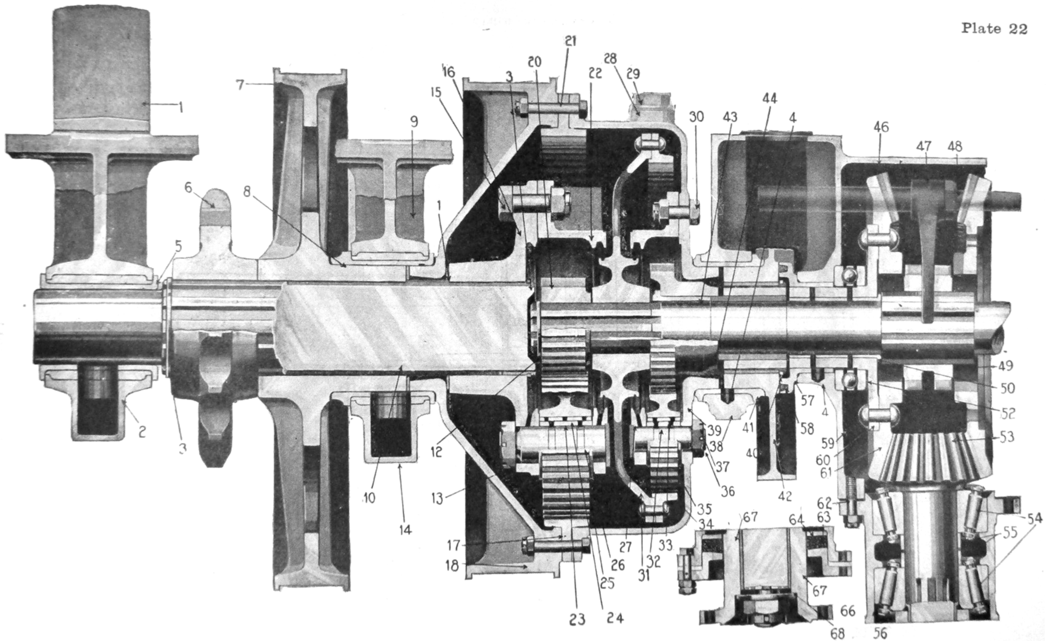
Transmission—Right half, sectional view
