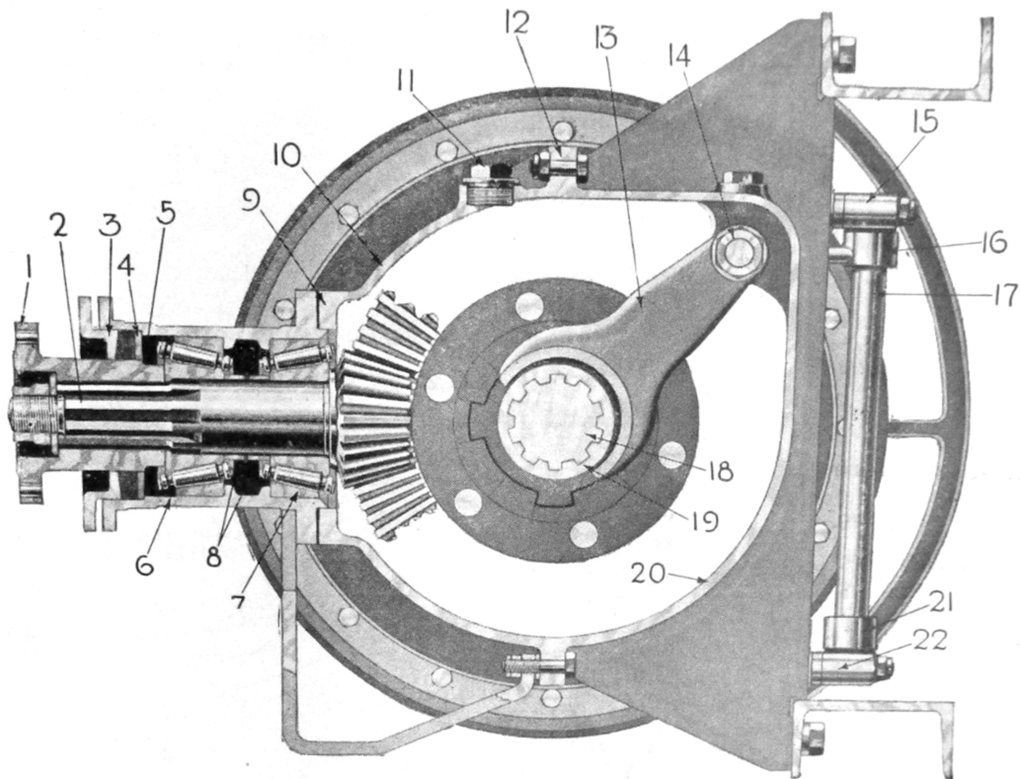
Bevel pinion drive—Assembled view
