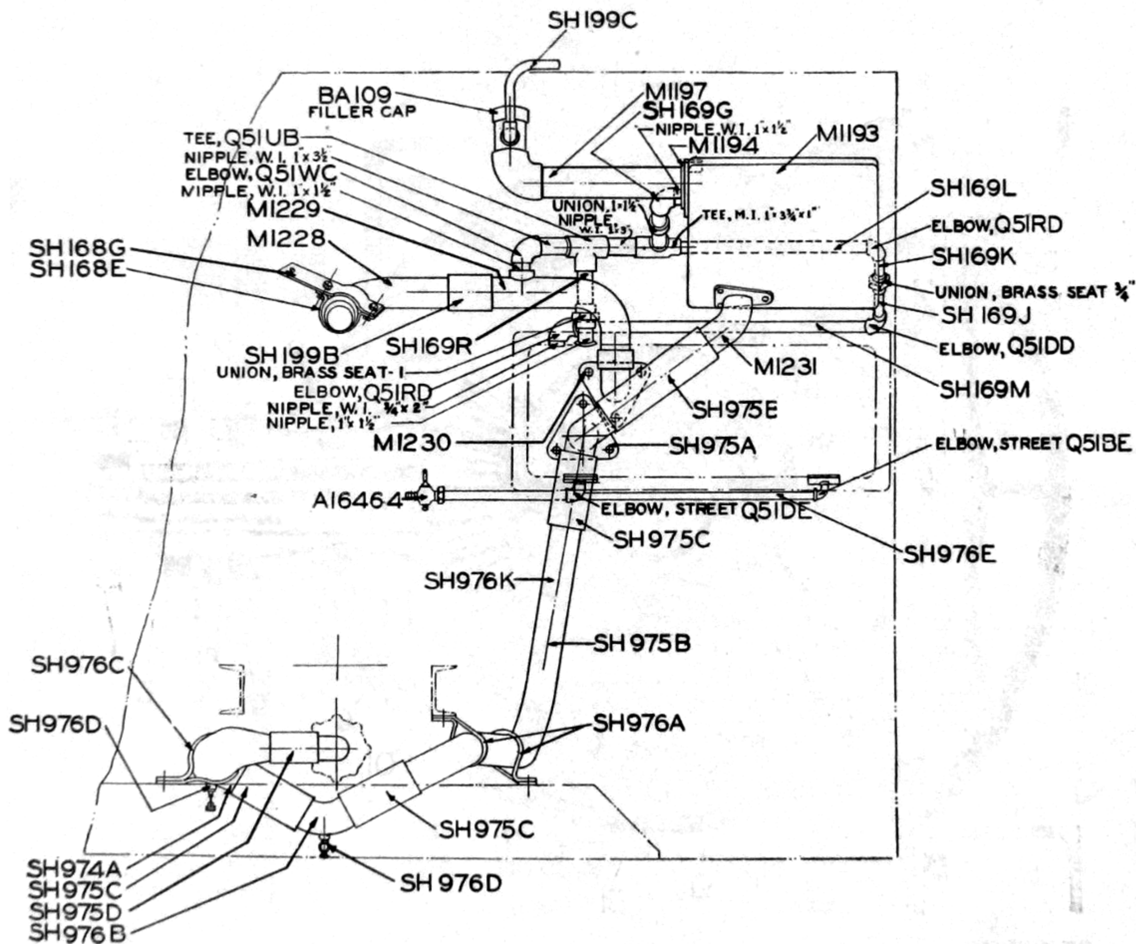
Radiator cooling system—Assembled view
