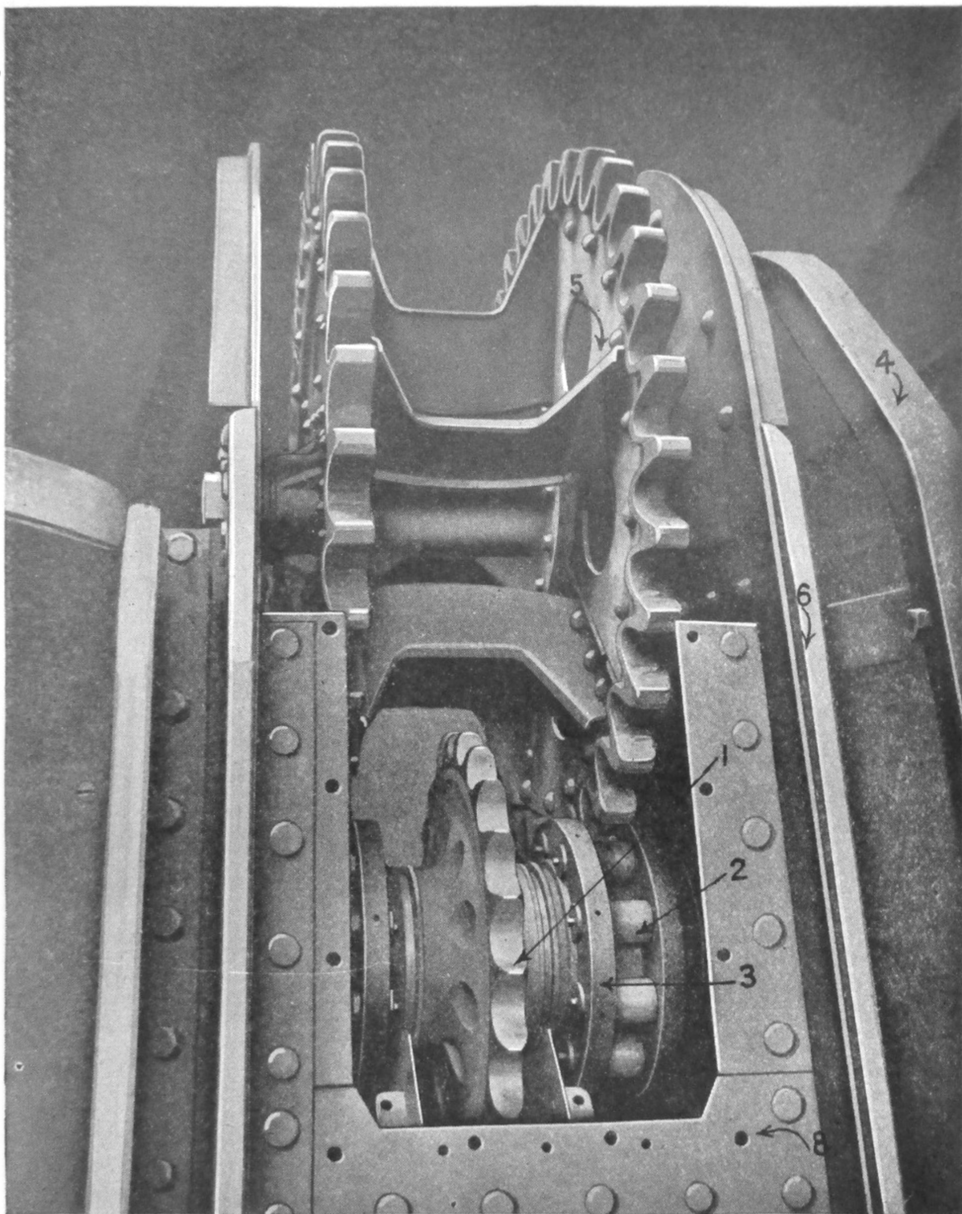
Roller pinion and track drive—Assembled view
