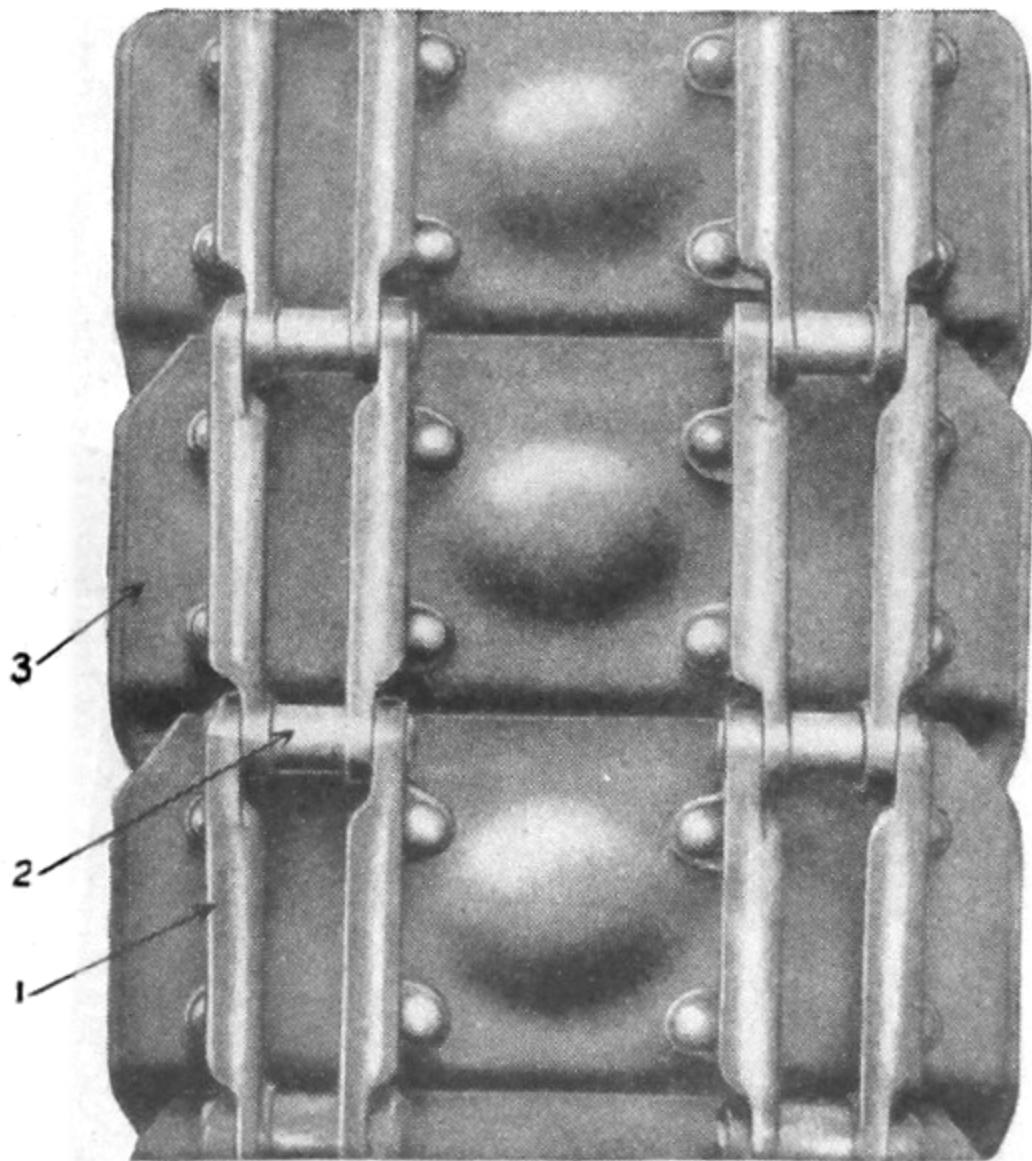
Track link—Assembled view
