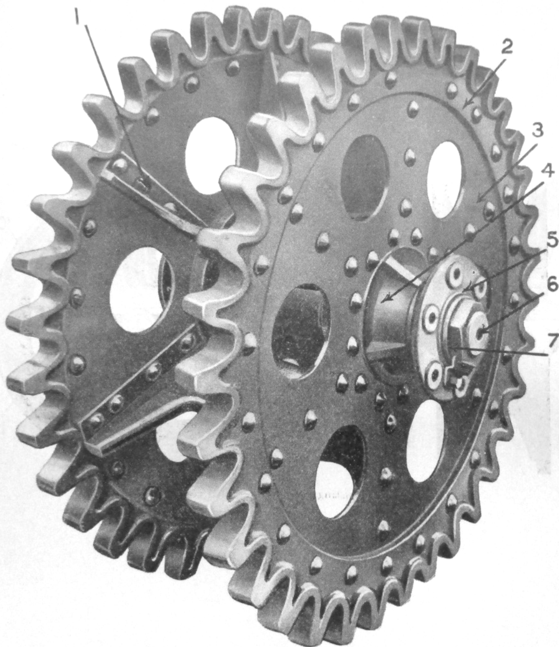
Track driving wheel—Assembled view
