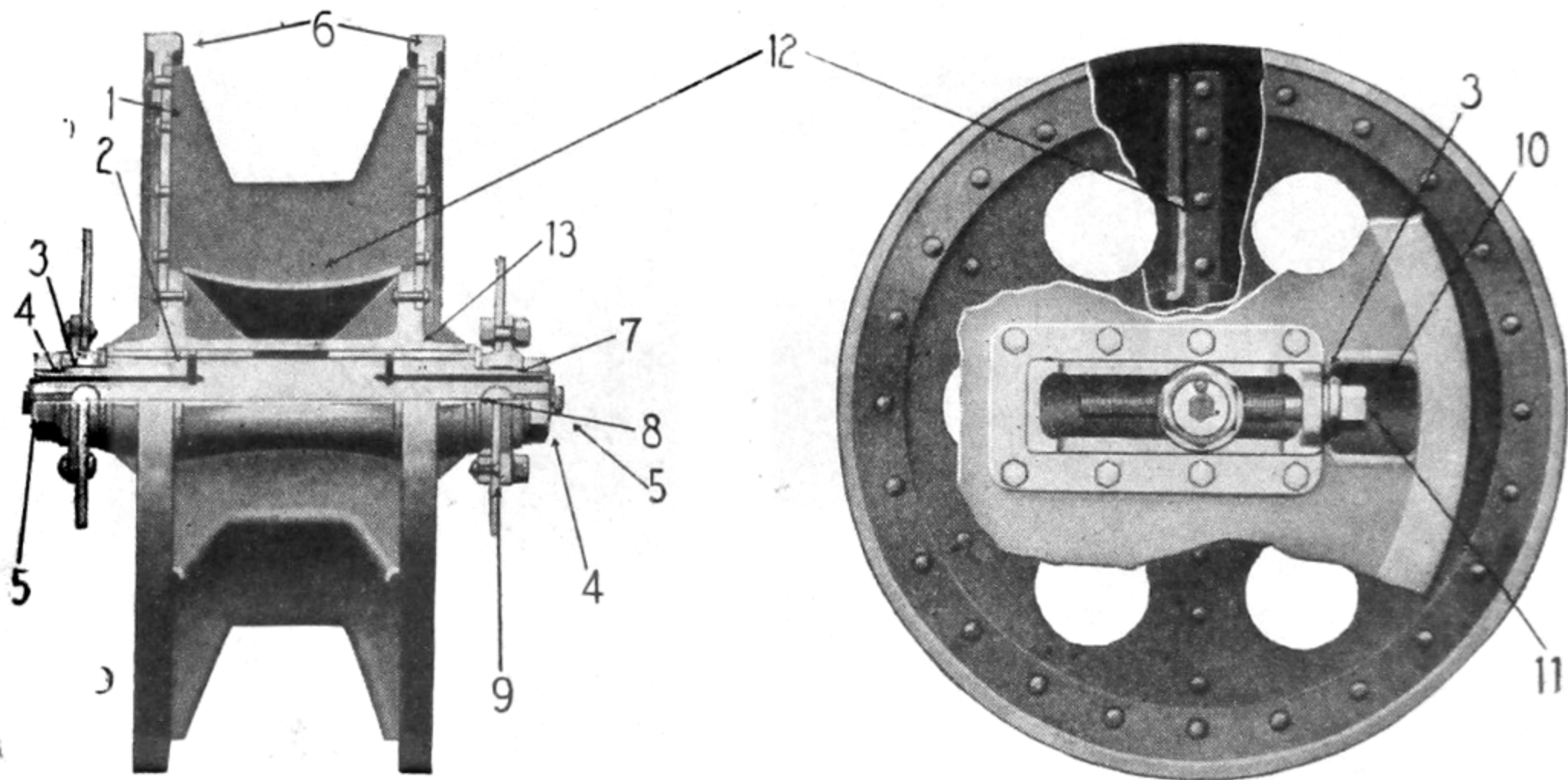
Track adjusting wheel—Assembled views
