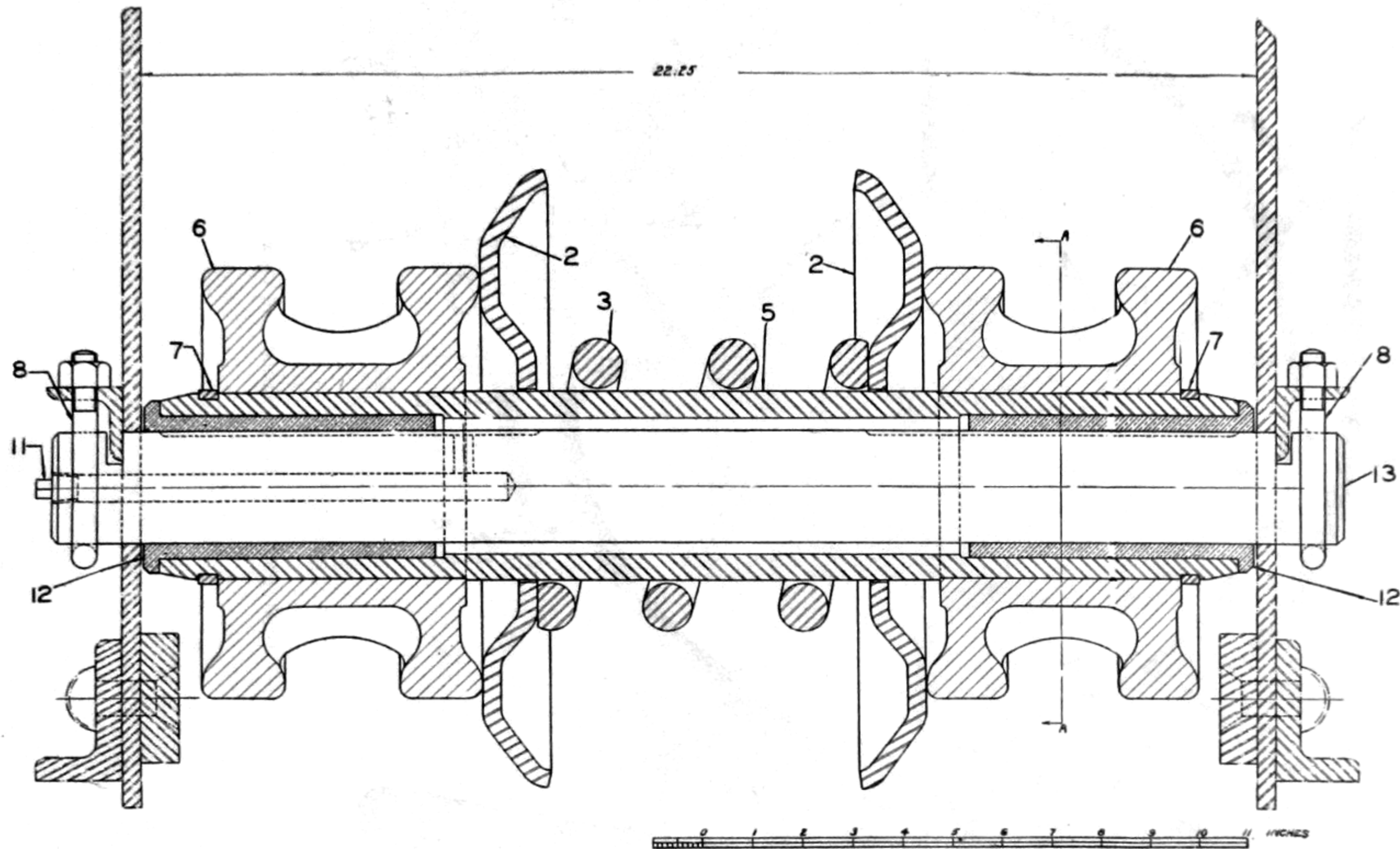
Track roller, with flanges—Assembled view
