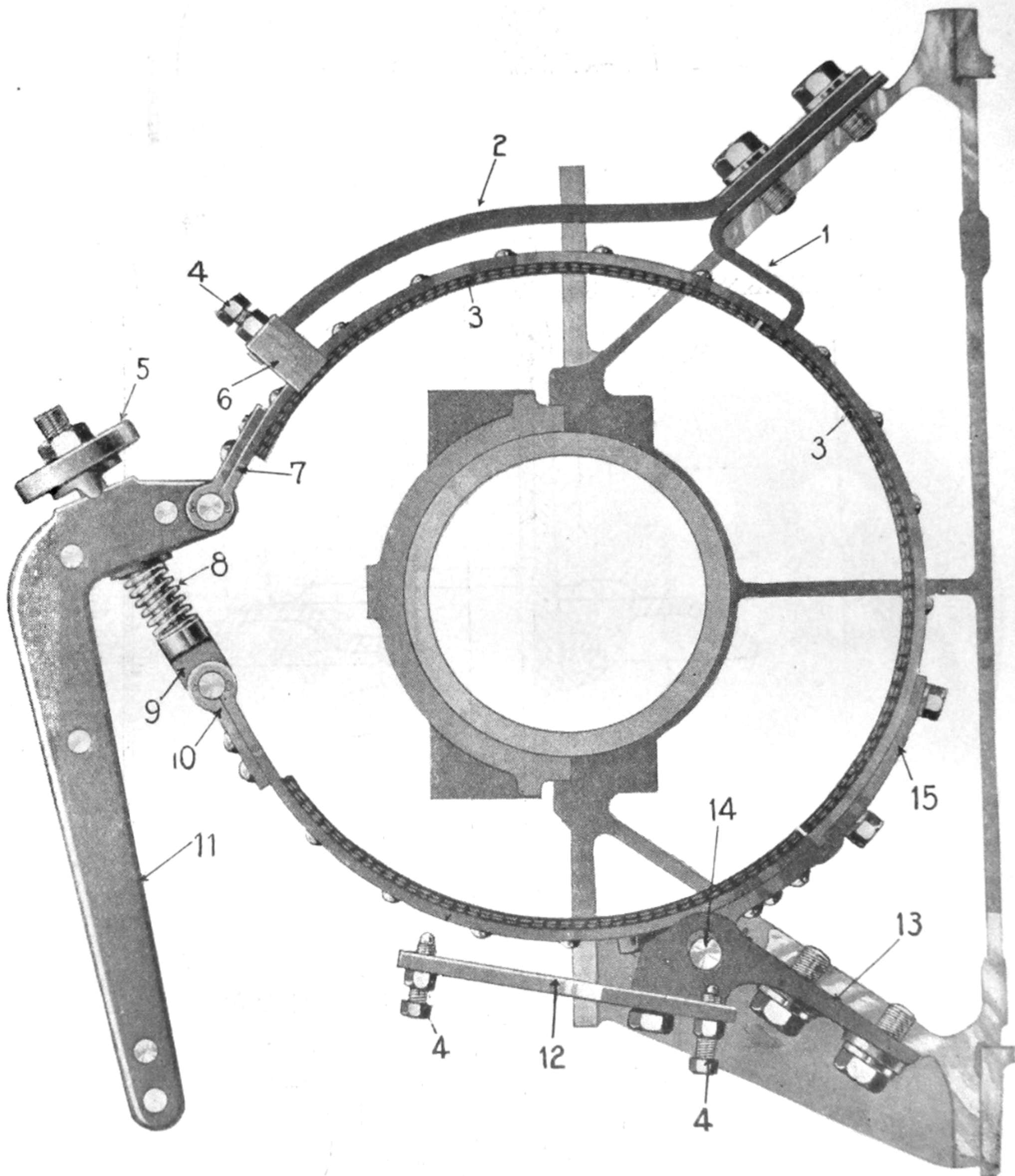
High speed brake band—Assembled view
