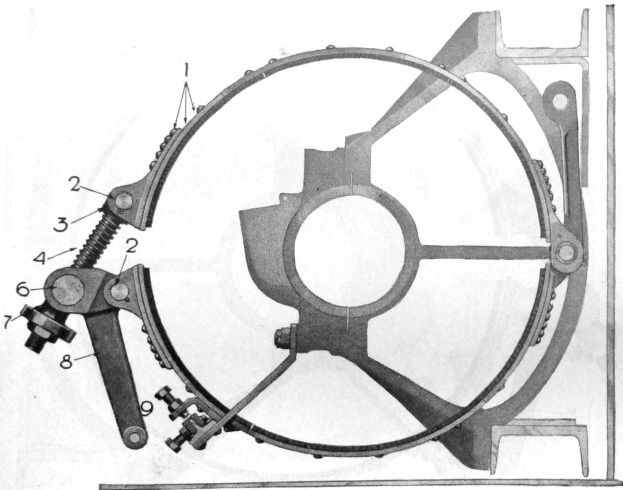
Track brake band—Assembled view
