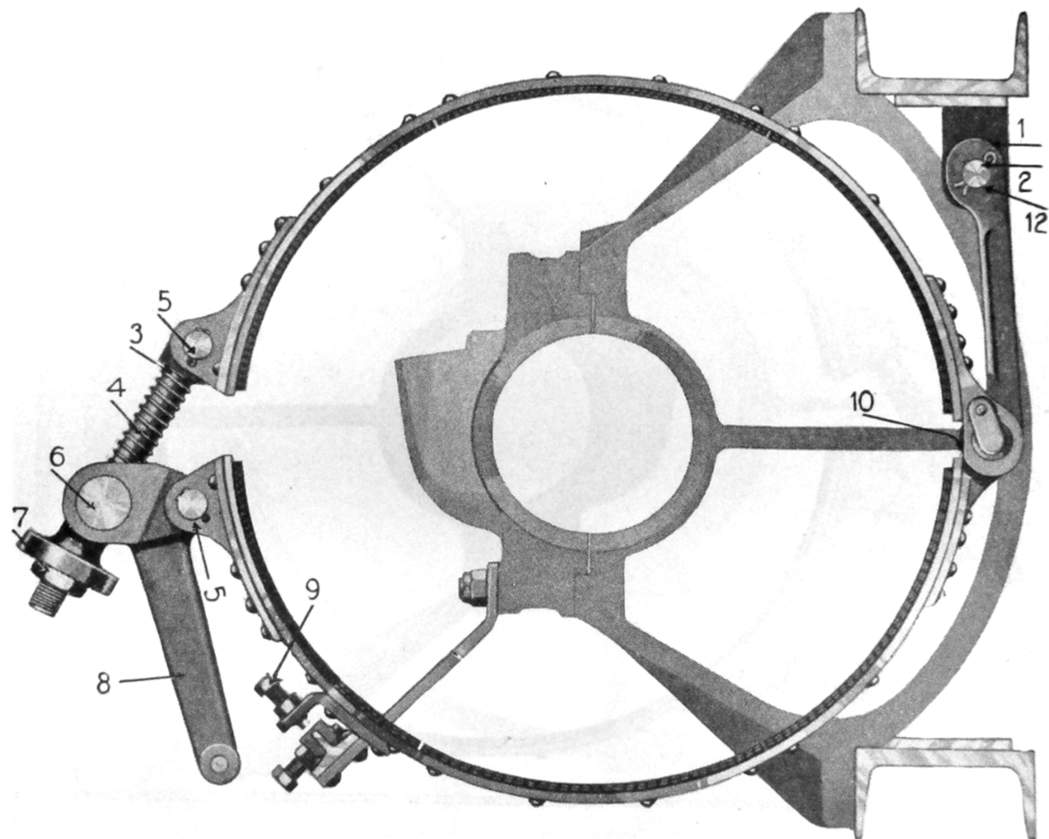
Low speed brake band—Assembled view
