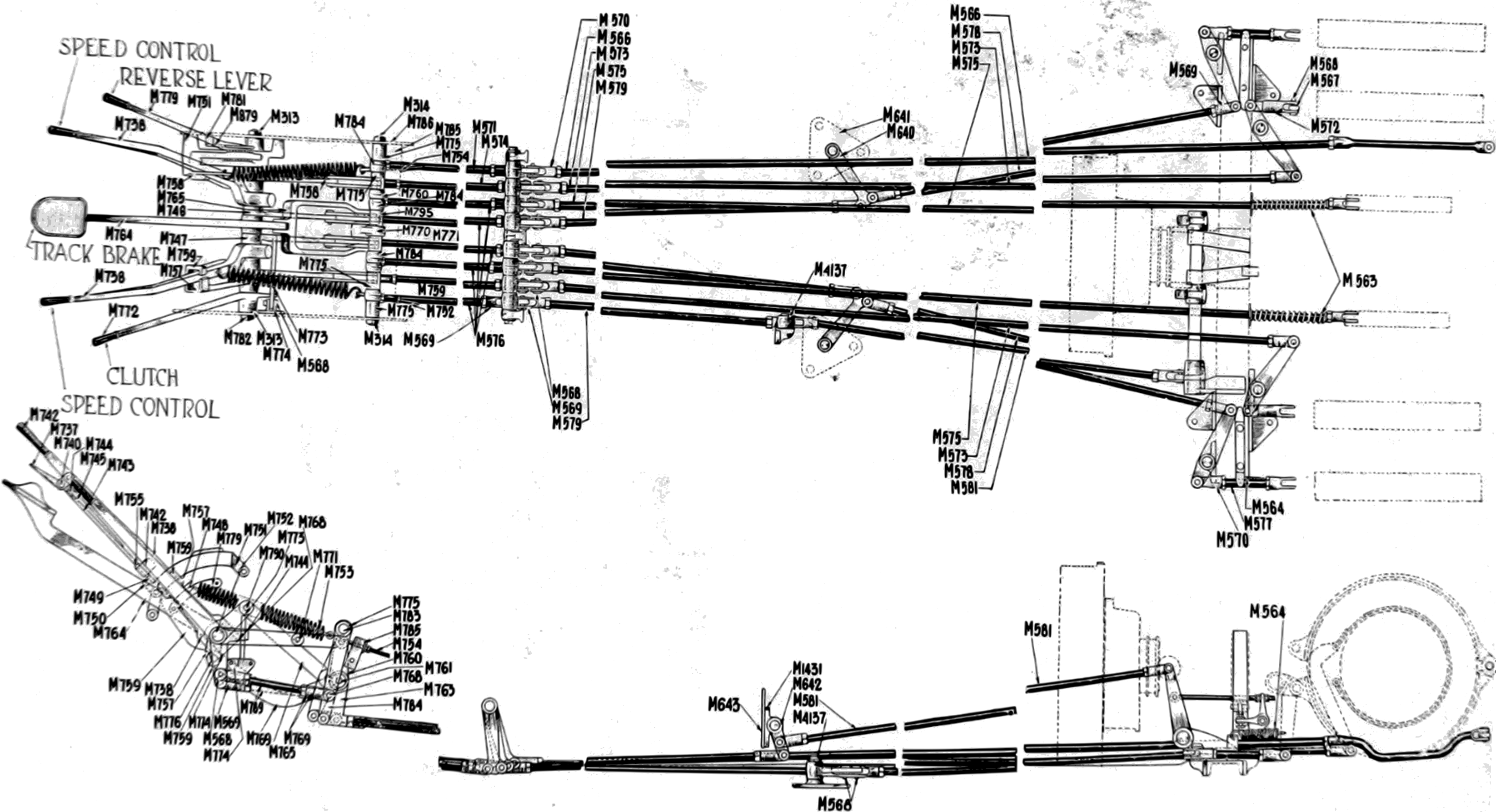
Control system—Assembled views
