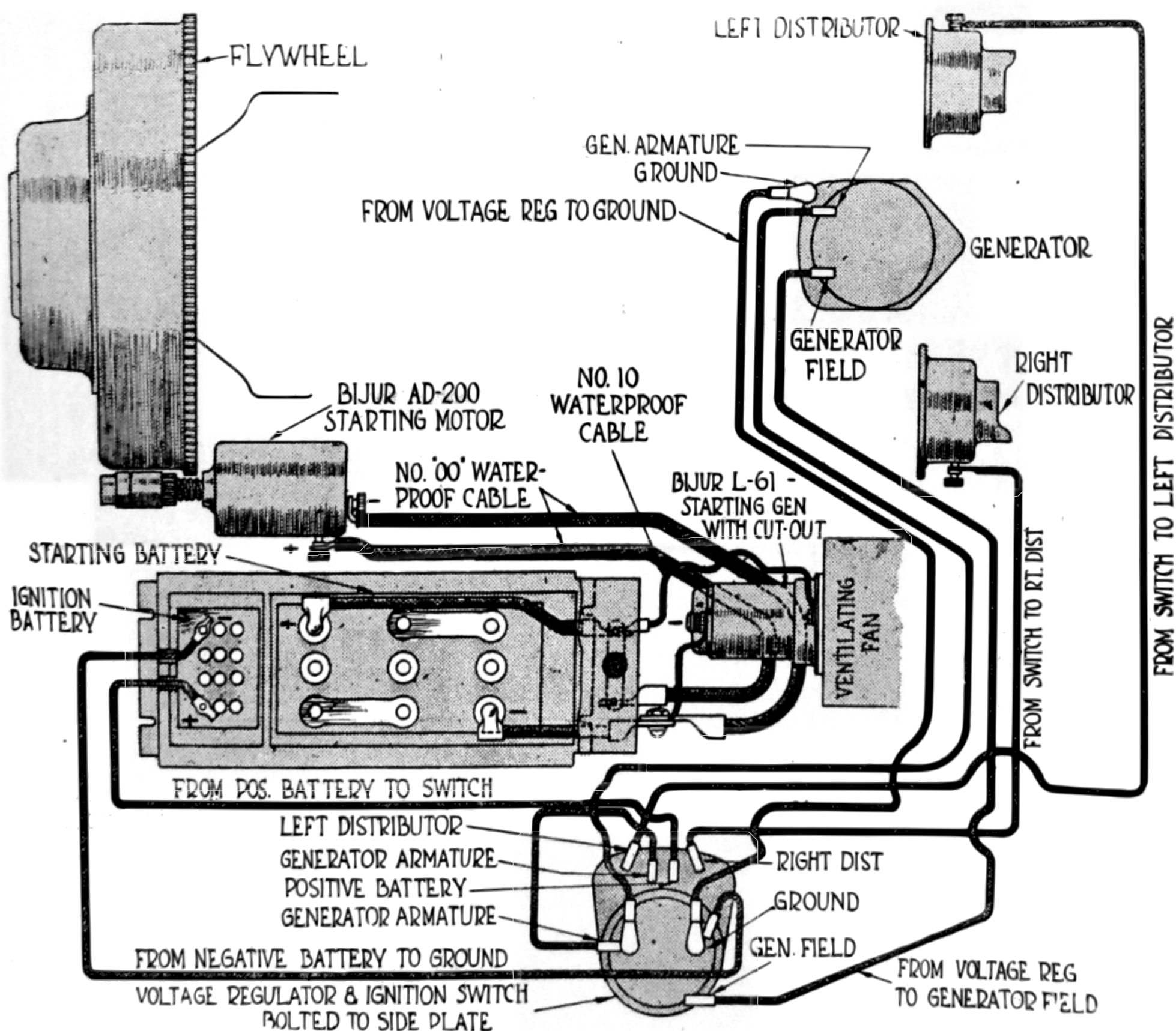
Schematic wiring diagram
