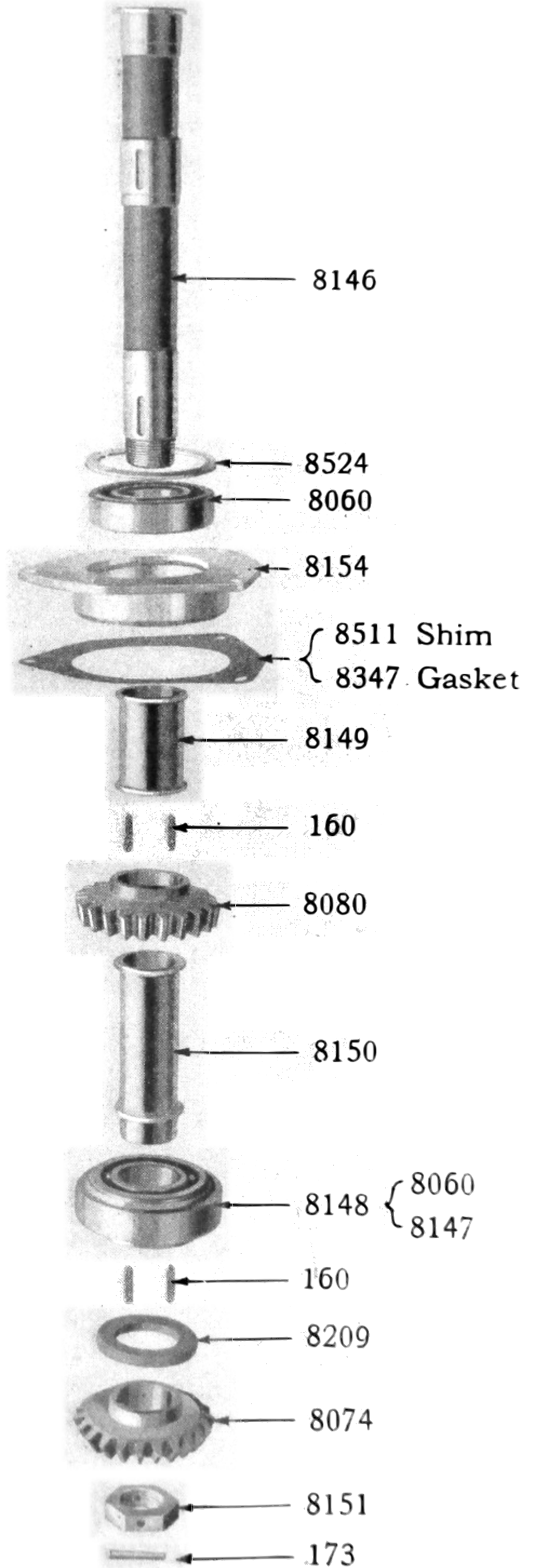
Generator drive shaft—Parts
