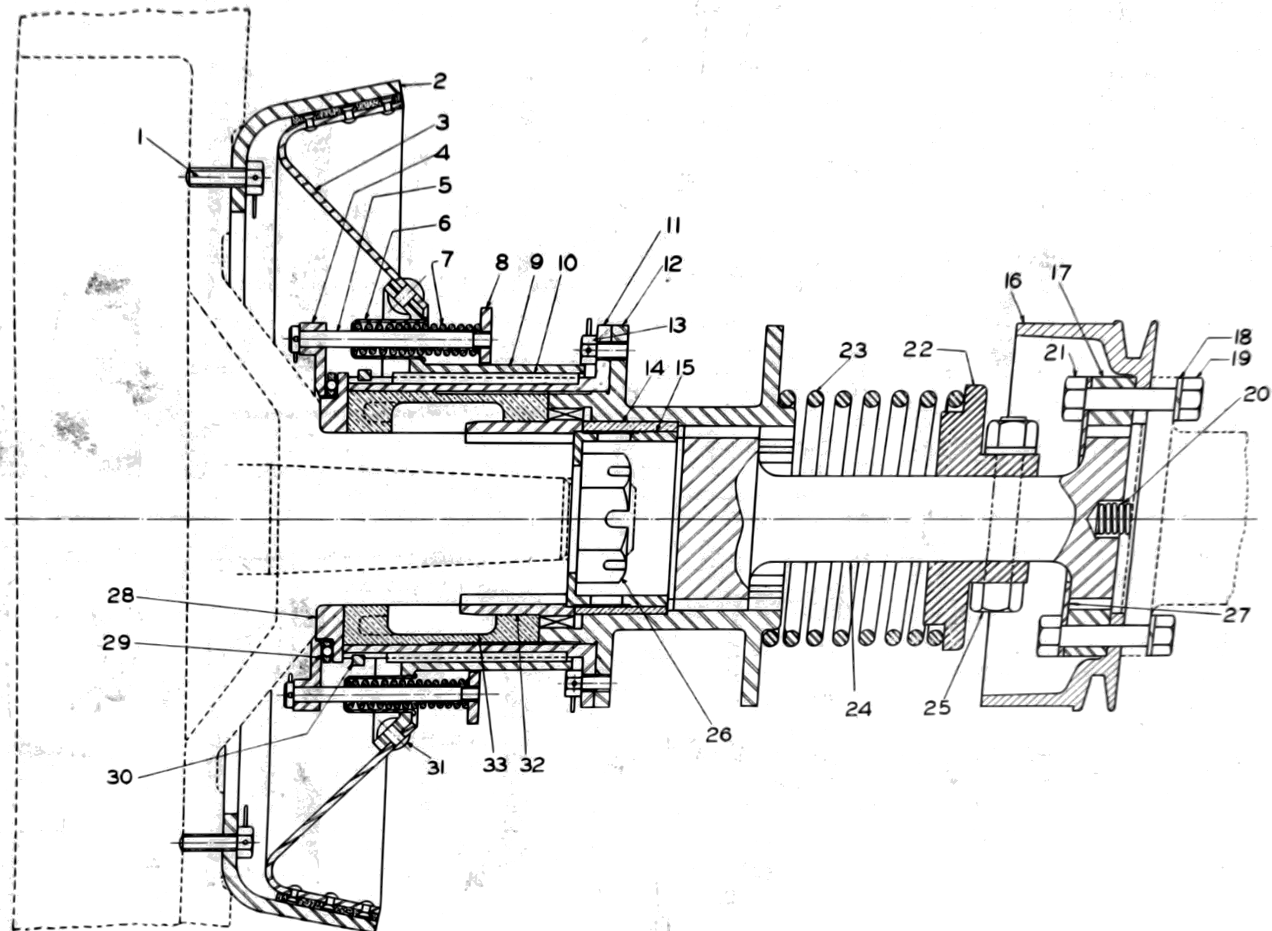
Clutch—Assembled view
