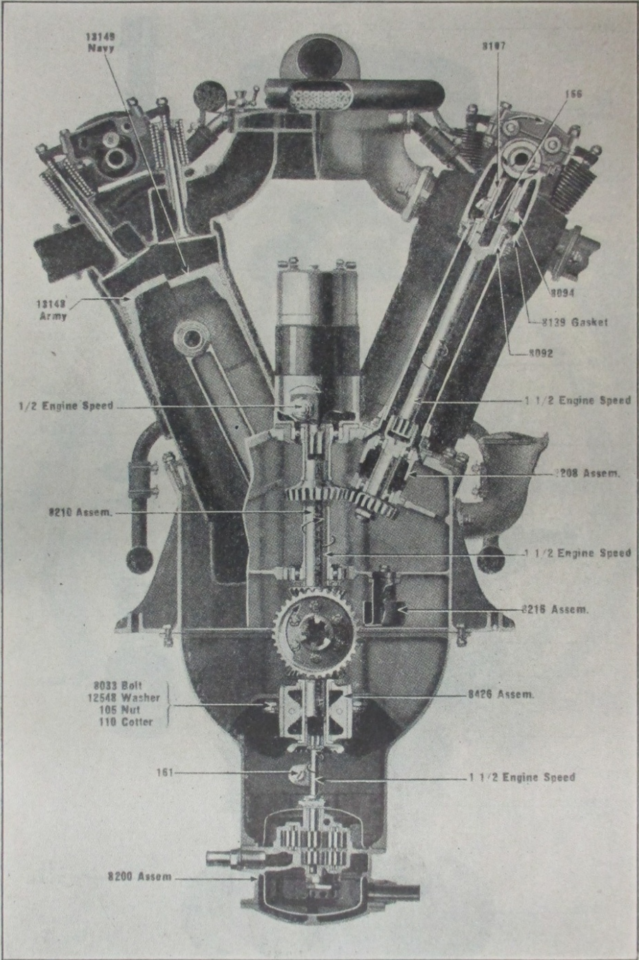
Liberty engine, transverse section—Assembled view
