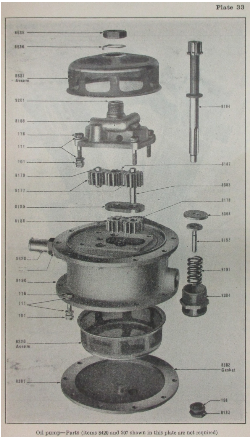
Oil pump—Parts (items 8420 and 207 shown in this plate are not required)
