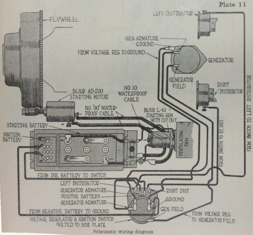
Schematic wiring diagram
