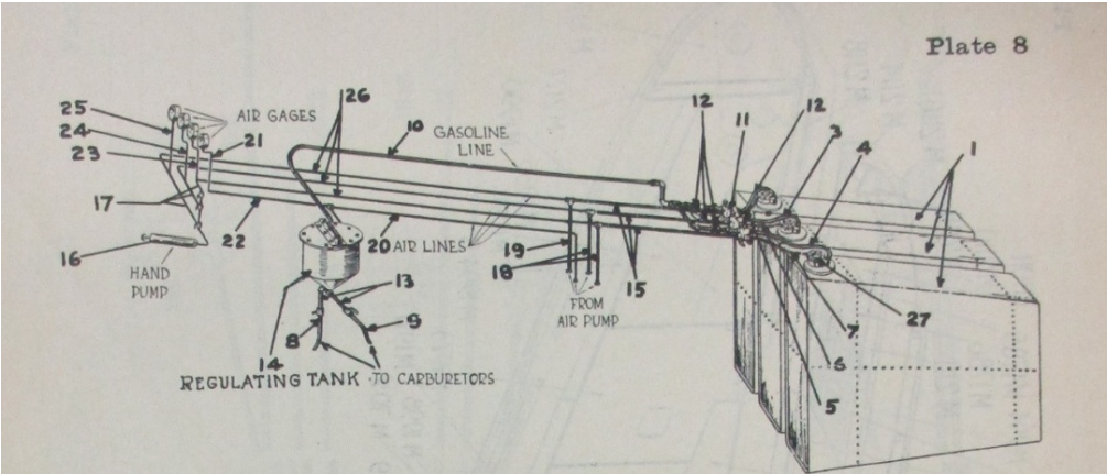
Gasoline tanks with pressure system—Assembled view
