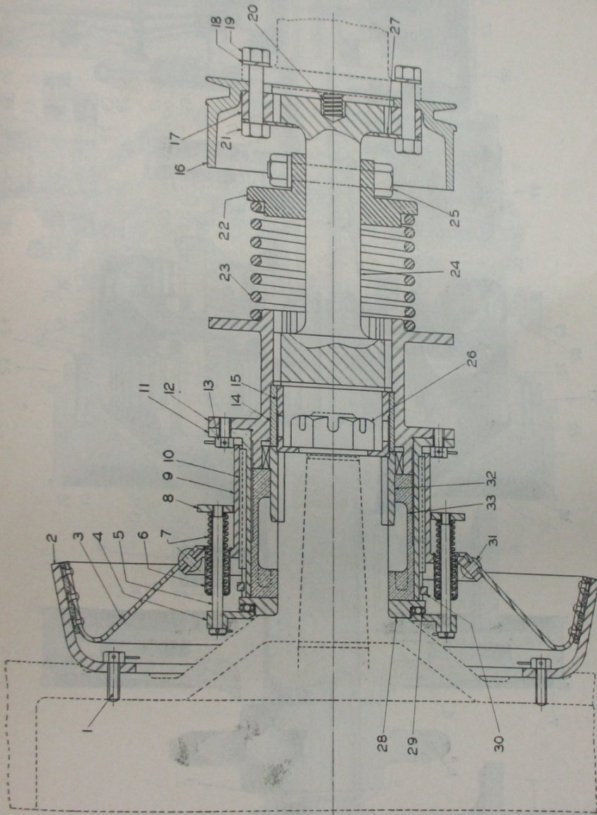
Clutch—Assembled view
