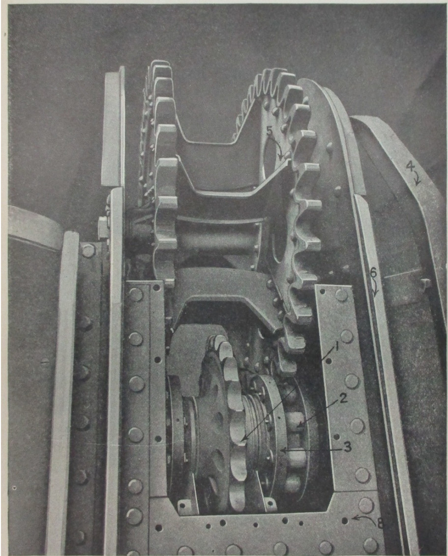
Roller pinion and track drive—Assembled view
