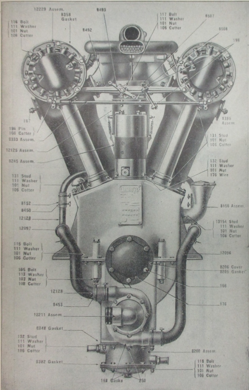
Liberty engine—Distributor end, assembled view. (Installation of governor eliminates the cover 8206)
