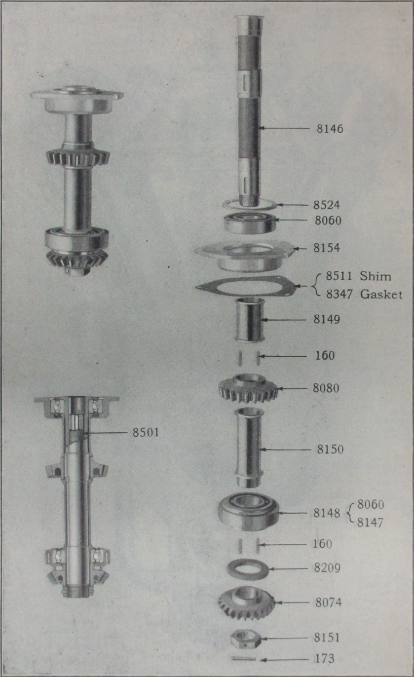
Generator drive shaft—Parts
