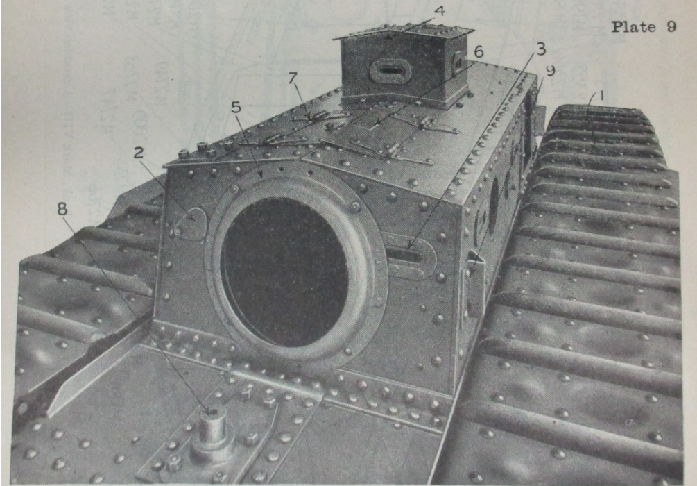
Main turret—Assembled view
