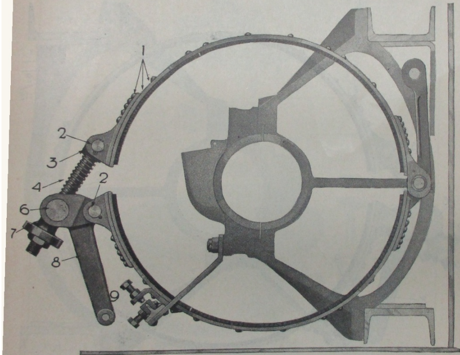
Track brake band—Assembled view
