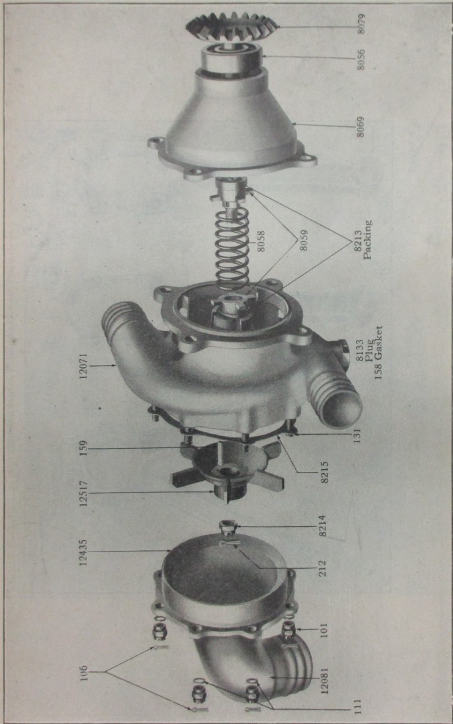
Water pump—Parts
