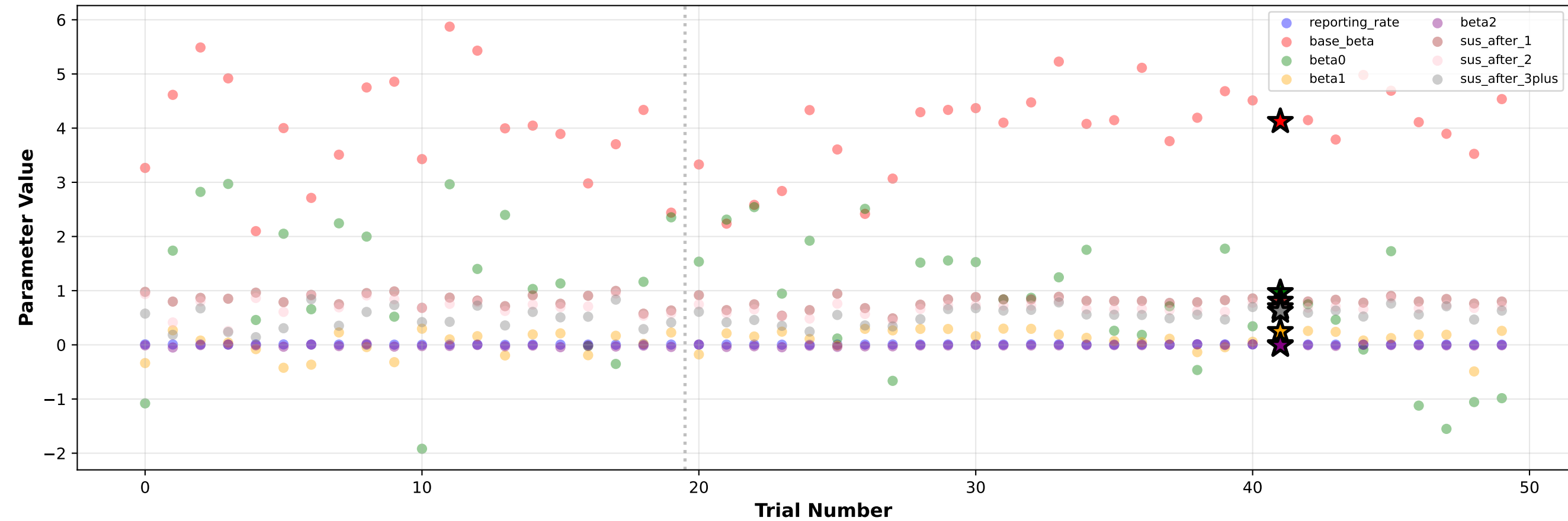
Parameter Values over Extended Calibration (★ = Best Trial #41)
