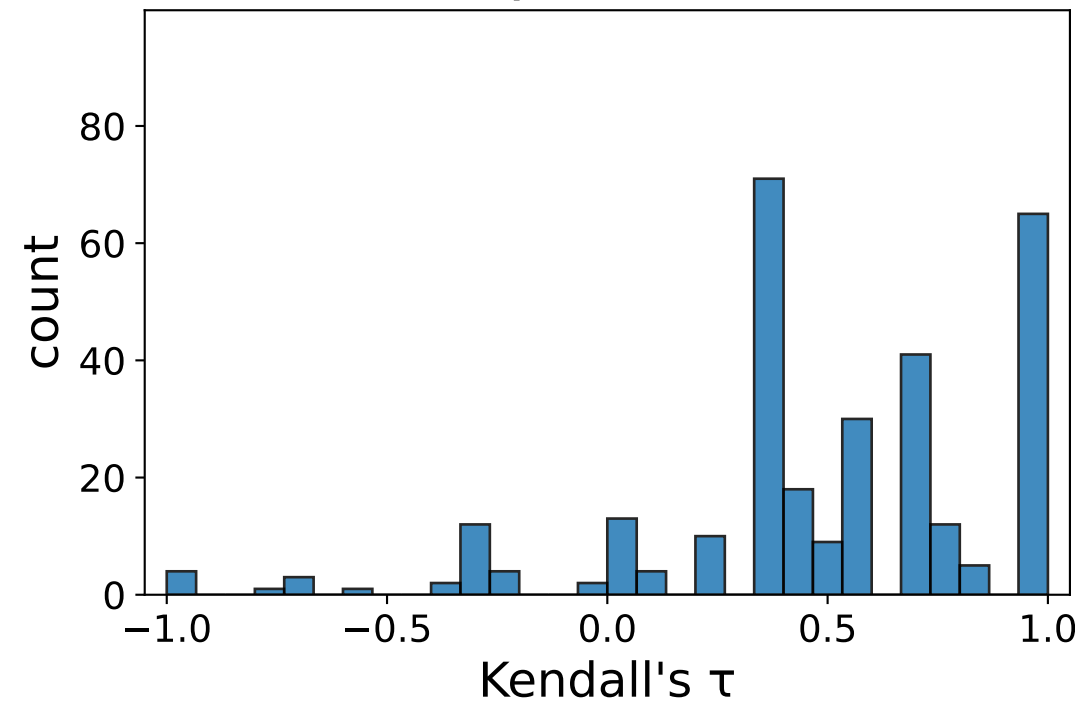
Human v.s. Qwen3-VL-4B-Instruct
