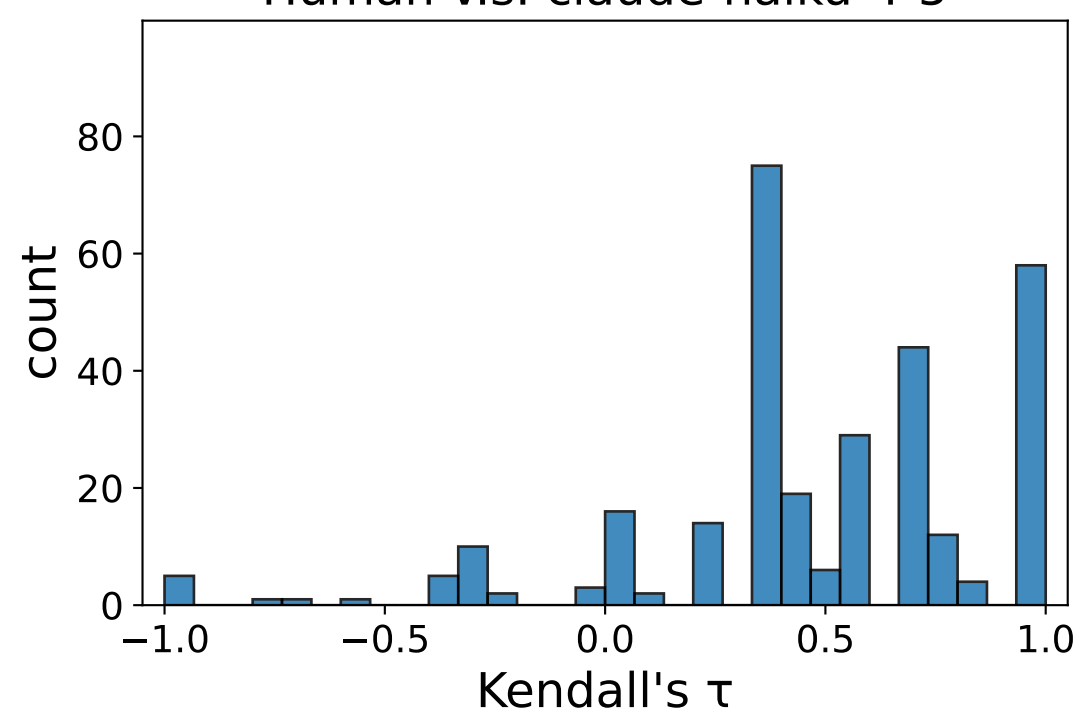
Human v.s. claude-haiku-4-5
