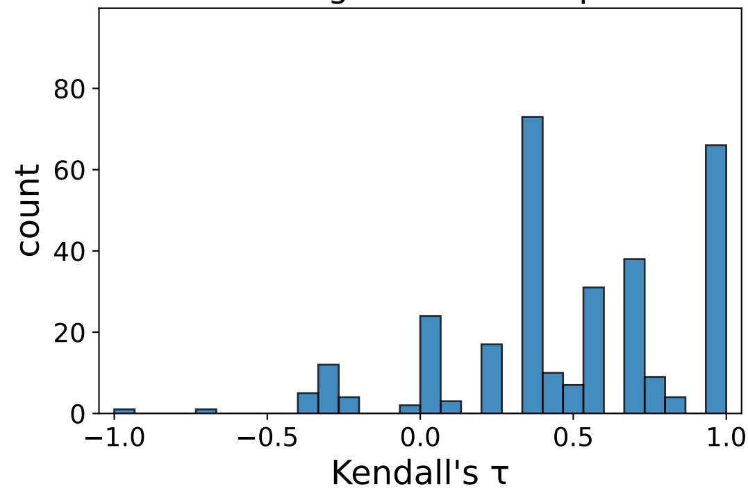
Human v.s. gemini-3-flash-preview
