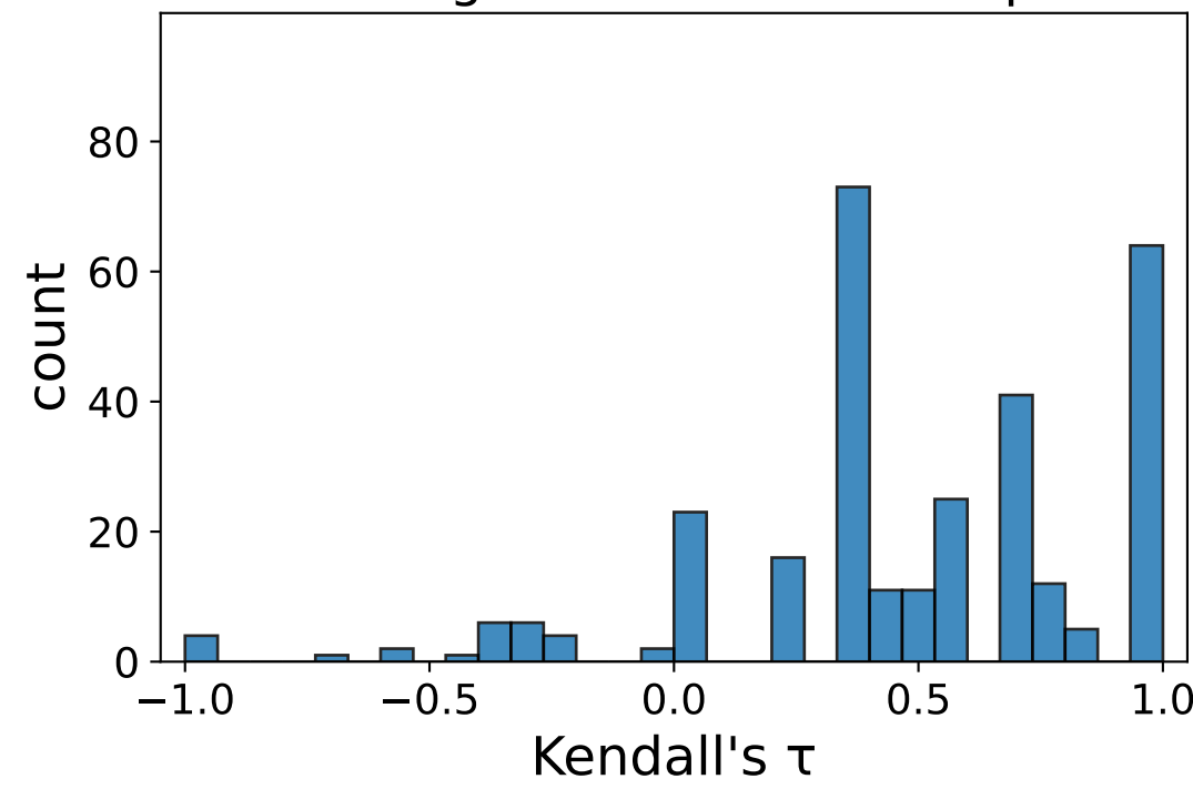
Human v.s. gemini-3.1-flash-lite-preview
