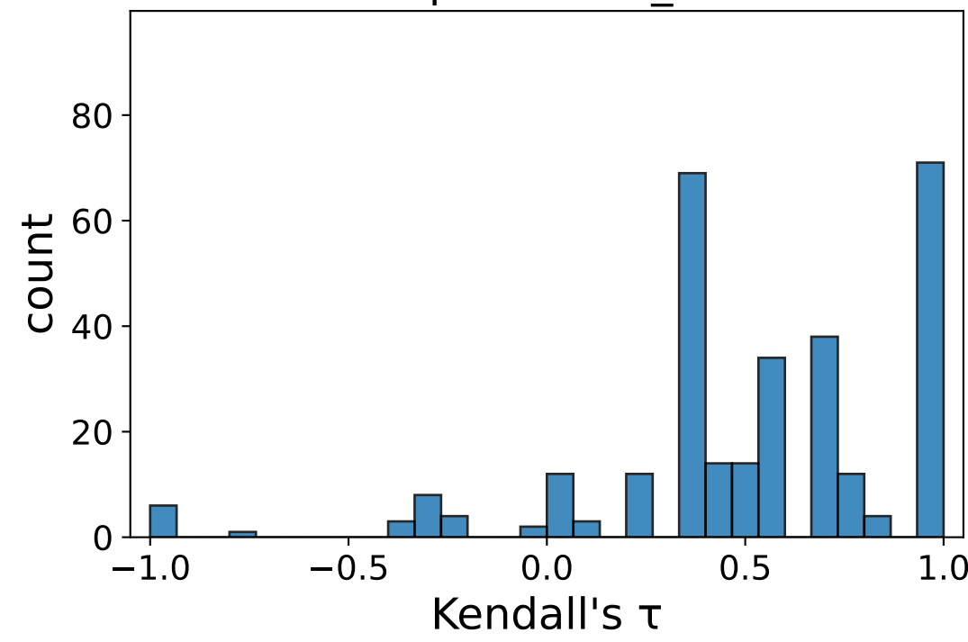
Human v.s. OpenGVLab_InternVL3-8B
