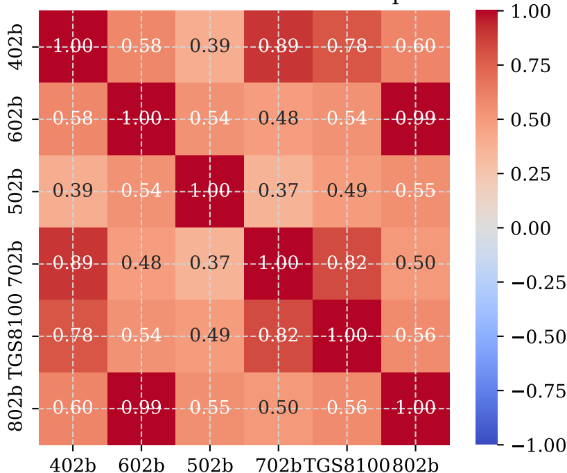
Sensor Correlation Heatmap
