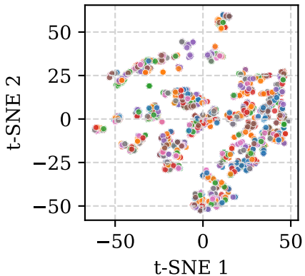
Perplexity: 30
