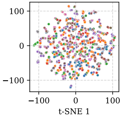
Perplexity: 5
