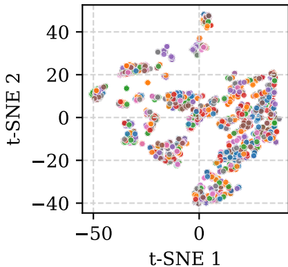
Perplexity: 50
