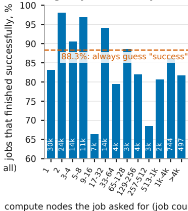
Fugaku jobs: will this job fail?
