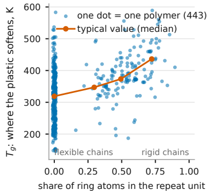
Polymers: softening point
