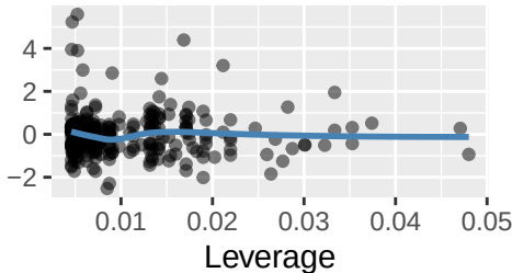
Residual vs. Leverage
