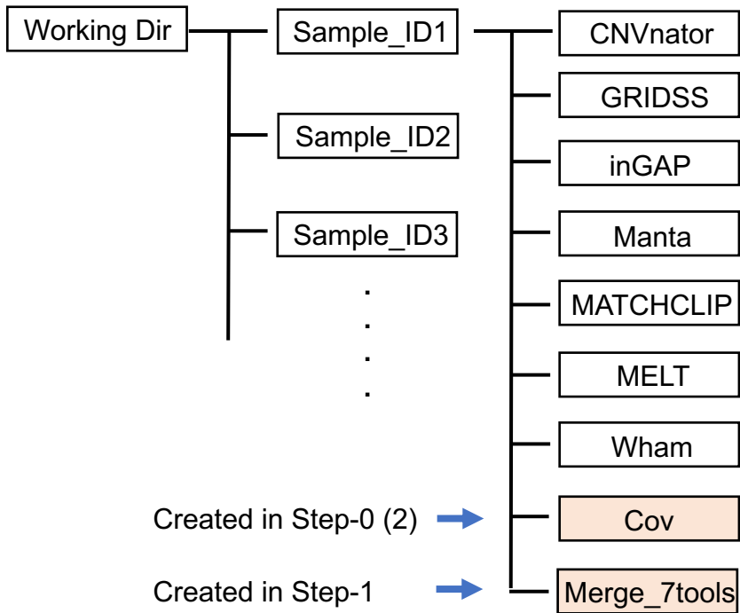
Directory structure used for MOPLine
