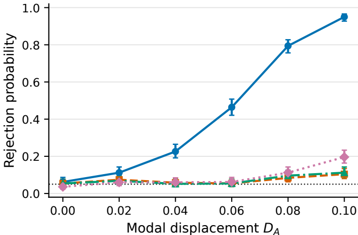
(a) Five-mode Student- t_5 , \lambda = 0
