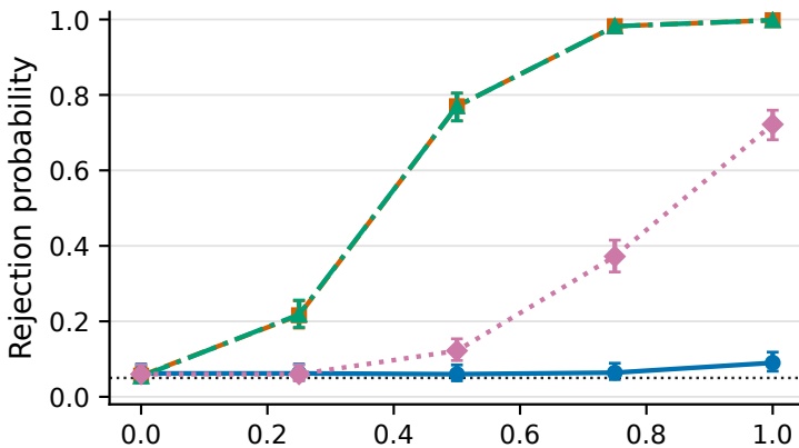
(c) Four-mode Gaussian: mass redistributed, modes fixed
