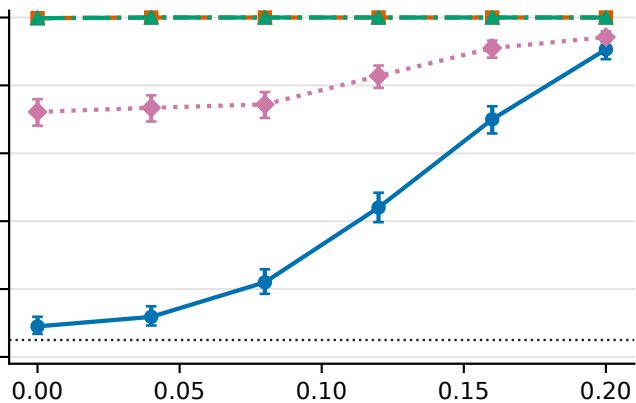
(d) Four-mode Gaussian: mass redistributed and modes moved
