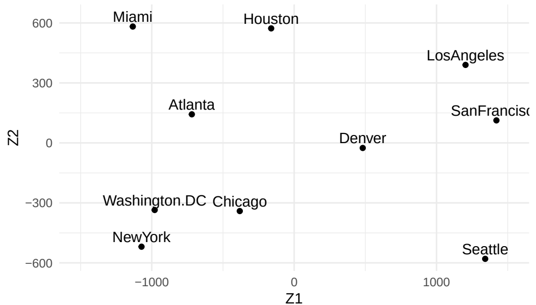
MDS plot of the UScitiesD data
