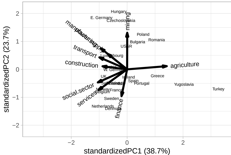
Biplot for the industries PCA
