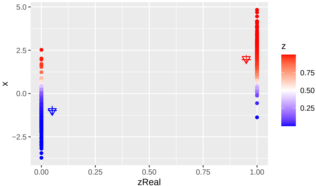
iteration 6 real mean (triangle), estimate mean (+)
