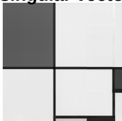
5 singular vectors
