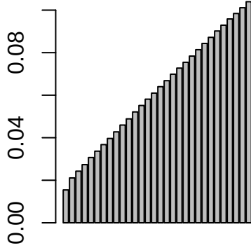
cummulative variance
