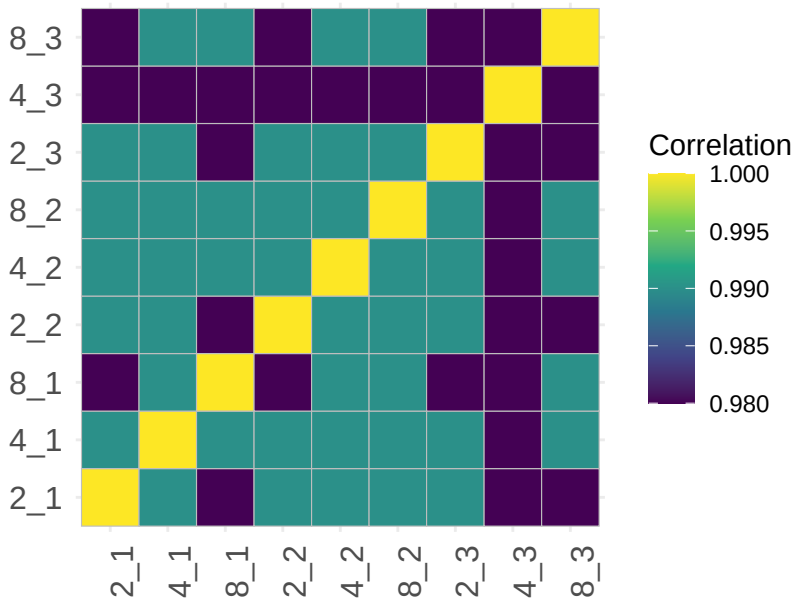
Correlation matrix
