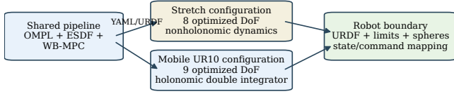
Fig. 2. The shared algorithm is specialized through robot profiles and an explicit platform boundary.
