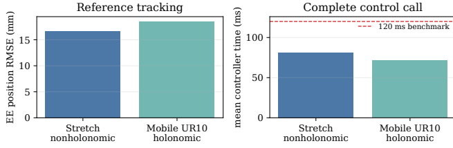
Fig. 4. Measured reference tracking and complete control-call time for the two configurations. Different geometry and tuning preclude a robot ranking.
