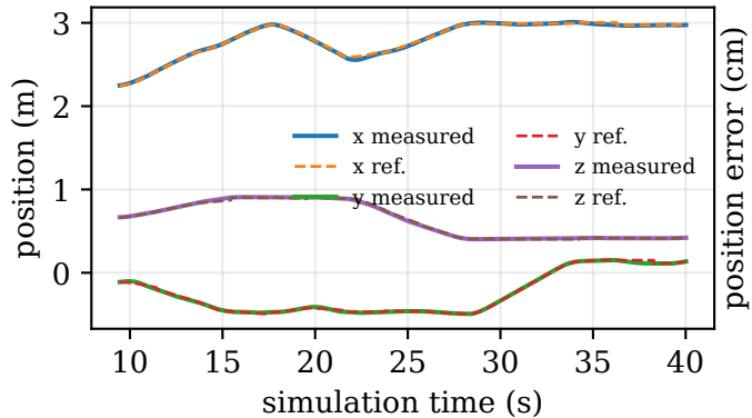
End-effector position
