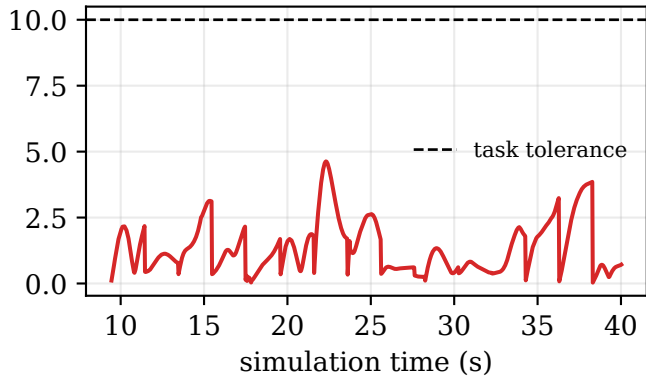
End-effector reference error
