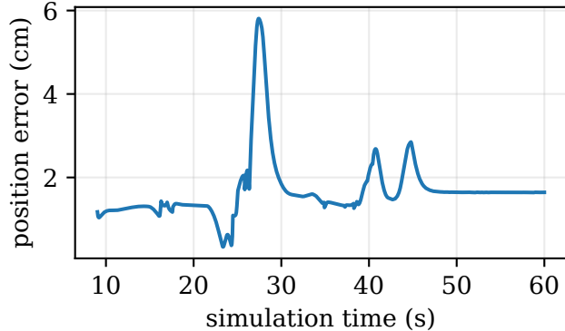
Mobile UR10: EE reference error
