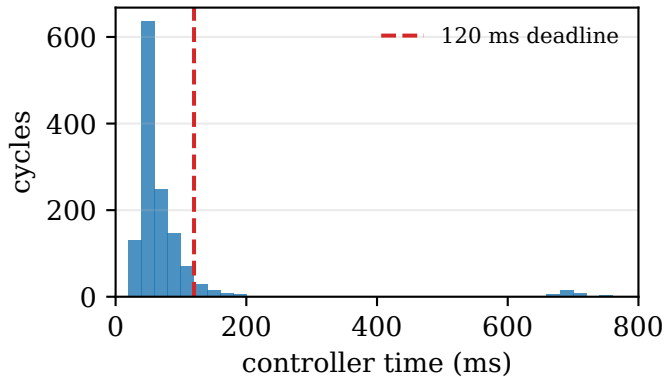
Runtime distribution
