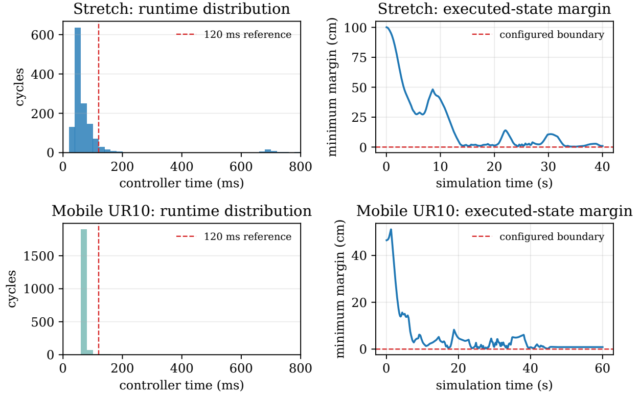
Fig. 6. Runtime distributions and minimum executed-state ESDF margins for Stretch (top) and mobile UR10 (bottom). The 120-ms line is a shared timing reference; the zero-margin line denotes each profile’s own configured collision boundary.
