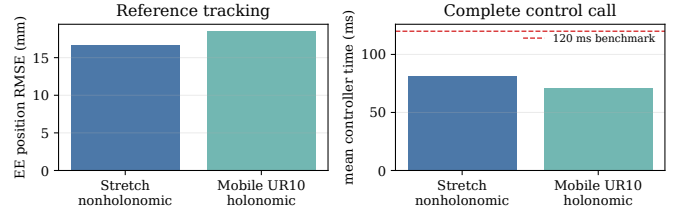
Fig. 4. Measured reference tracking and complete control-call time for the two configurations. Different geometry and tuning preclude a robot ranking.
