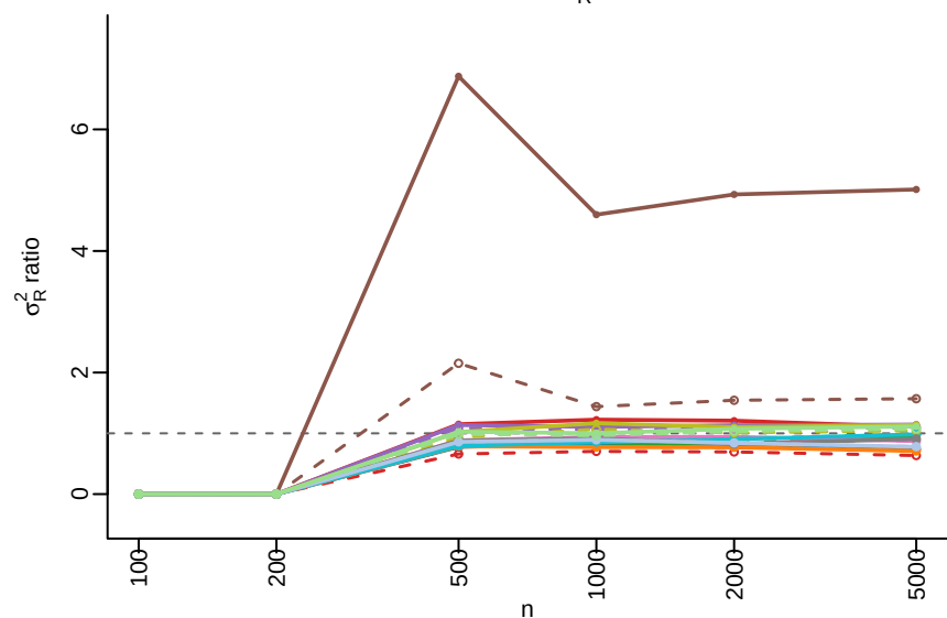
Parametric GLM: \sigma_R^2 calibration
