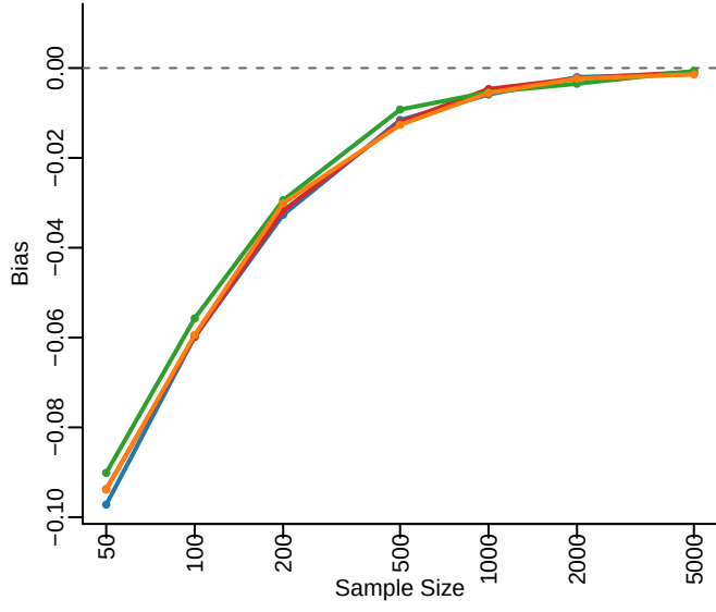
smoker: S=1.310
