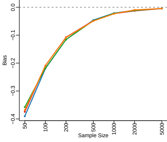
region: S=0.117
