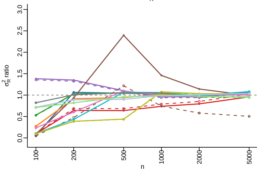
Robust GLM: \sigma_R^2 calibration
