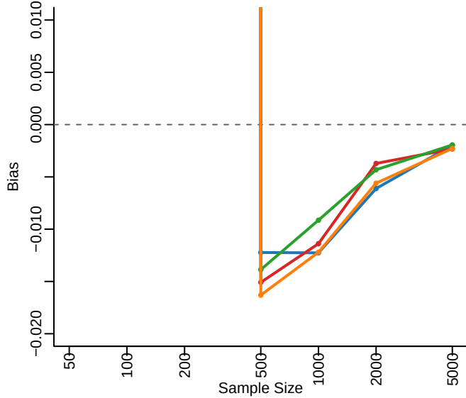
smoker: S=0.413
