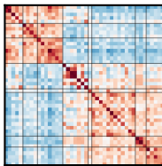
REPRESENT
