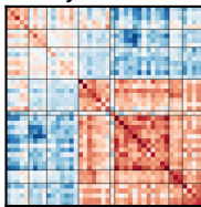
JUDGE
