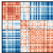
SELF
