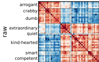
HUMAN
