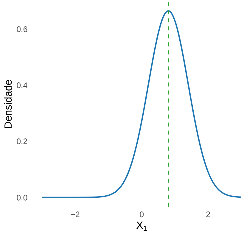
X_1 \mid X_2 = 1
