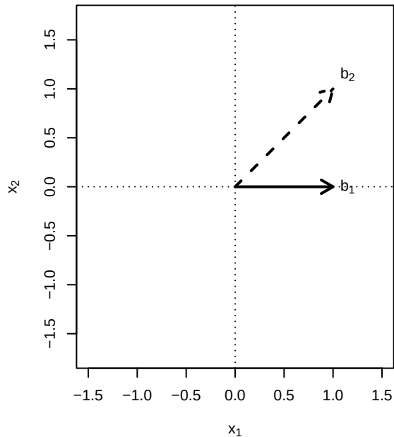
Base oblua
